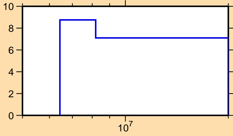
\Delta\sigma/\sigma vs. E for ^{176}\text{Ta}(n,\text{nonel.})
