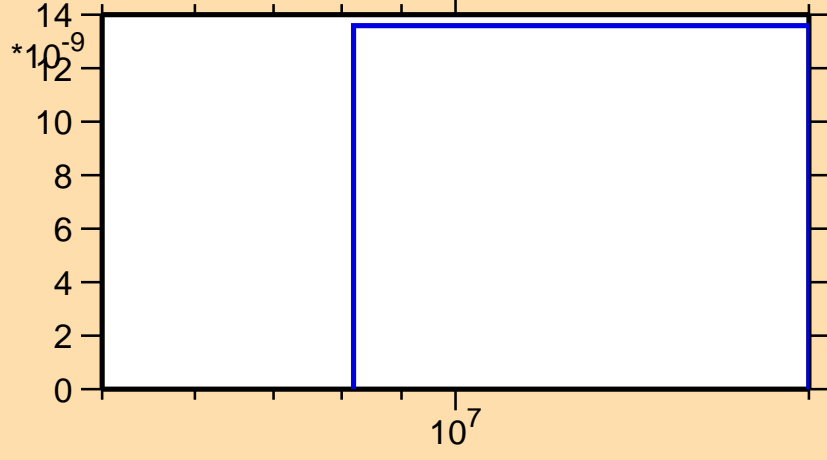
\sigma vs. E for ^{176}\text{Ta}(n,nt)
