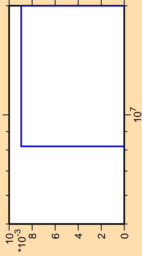
\Delta\sigma/\sigma vs. E for ^{176}\text{Ta}(n,\text{pt})
