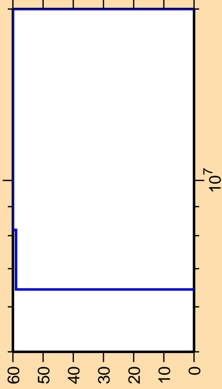
\Delta\sigma/\sigma vs. E for ^{176}\text{Ta}(n,n\text{cont.})
