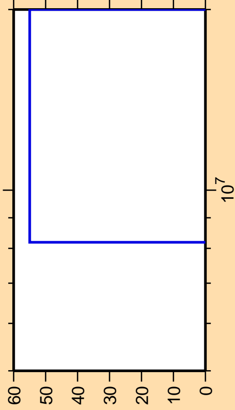
\Delta\sigma/\sigma vs. E for ^{176}\text{Ta}(n,3n)
