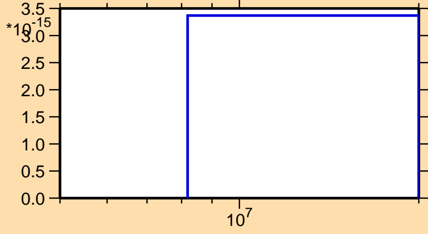
\sigma vs. E for ^{176}\text{Ta}(n,pd)
