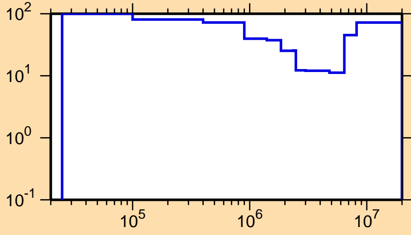
\Delta\sigma/\sigma vs. E for ^{176}\text{Ta}(n,\text{inel.})
