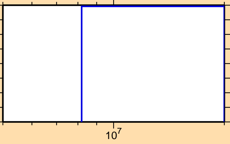
\sigma vs. E for ^{176}\text{Ta}(\text{mt } 34)
