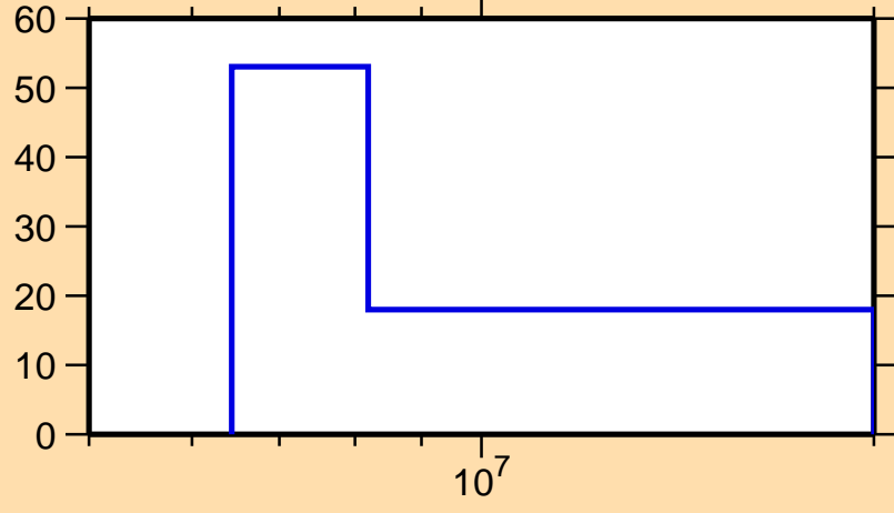
\Delta\sigma/\sigma vs. E for ^{176}\text{Ta}(n,2n)
