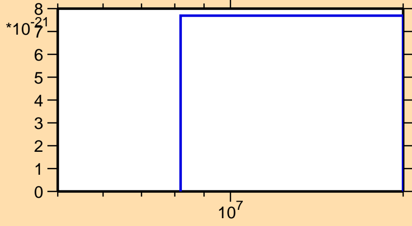
\sigma vs. E for ^{176}\text{Ta} (mt 42)
