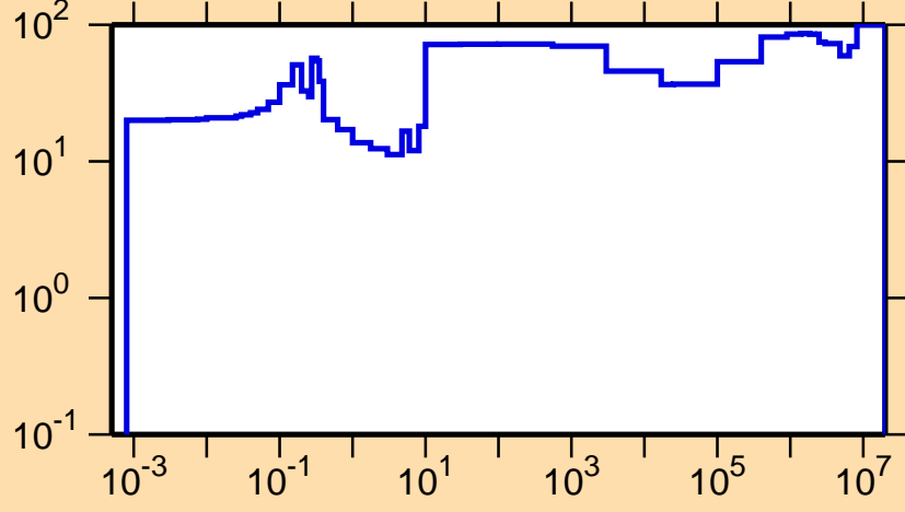
\Delta\sigma/\sigma vs. E for ^{176}\text{Ta}(n,\gamma)
