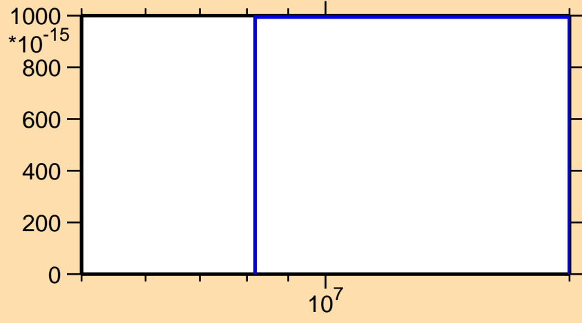
\sigma vs. E for ^{176}\text{Ta} (mt 45)
