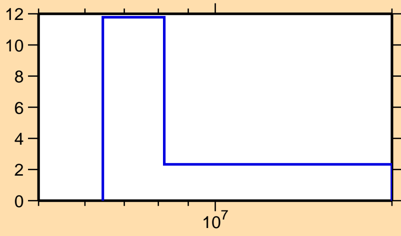
\Delta\sigma/\sigma vs. E for ^{176}\text{Ta}(n,\text{tot.})
