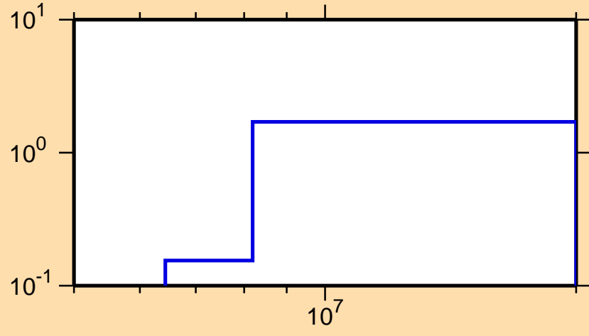
\sigma vs. E for ^{176}\text{Ta}(n,2n)
