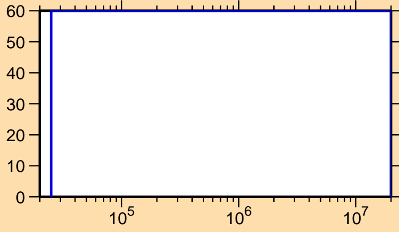
\Delta\sigma/\sigma vs. E for ^{176}\text{Ta}(n,n_1)
