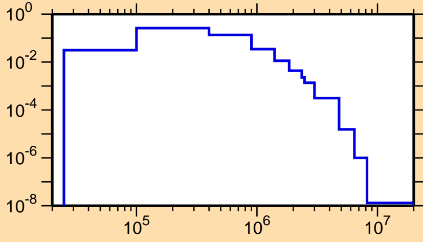
\sigma vs. E for ^{176}\text{Ta}(n,n_2)
