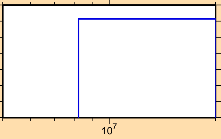
\sigma vs. E for ^{176}\text{Ta}(n,3n)
