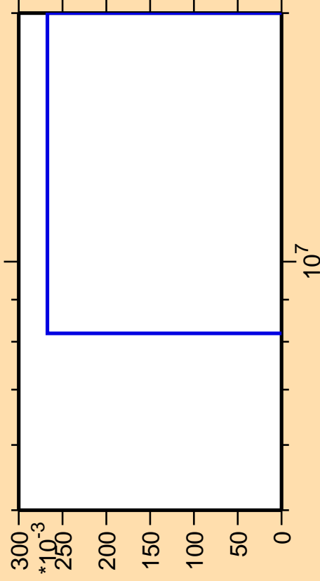
\Delta\sigma/\sigma vs. E for ^{176}\text{Ta}(\text{mt } 34)
