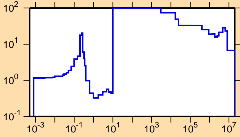
\Delta\sigma/\sigma vs. E for ^{176}\text{Ta}(n,\text{el.})
