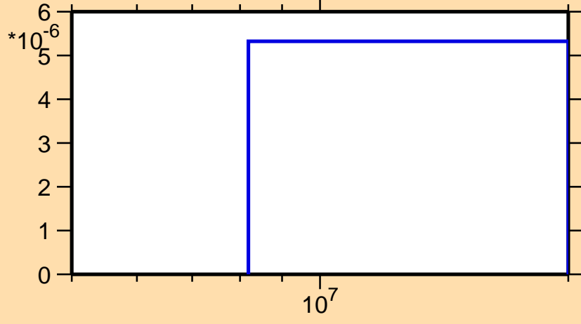
\sigma vs. E for ^{176}\text{Ta}(n,2np)
