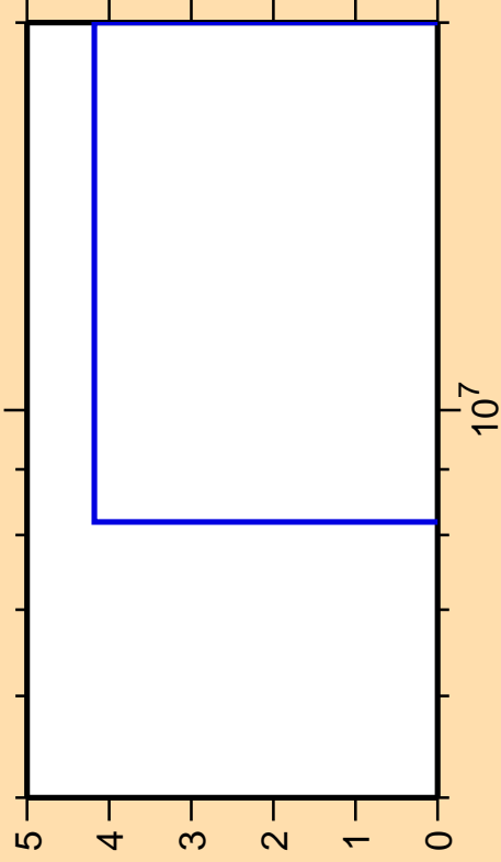
\Delta\sigma/\sigma vs. E for ^{176}\text{Ta}(\text{mt117})
