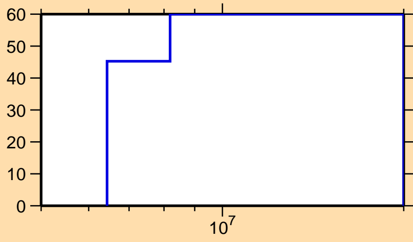
\Delta\sigma/\sigma vs. E for ^{176}\text{Ta}(n,\text{inel.})
