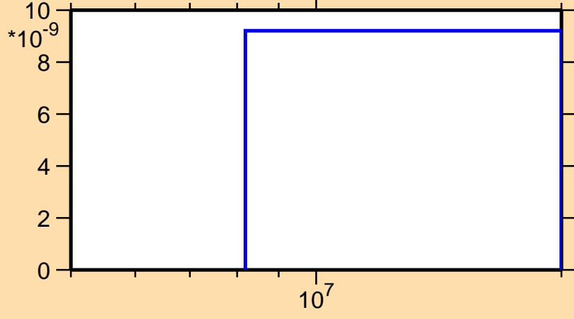
\sigma vs. E for ^{176}\text{Ta}(n,\text{He3})
