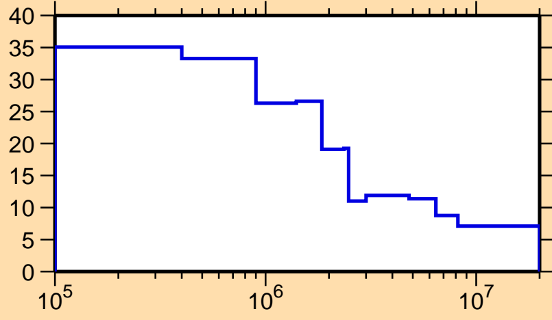
\Delta\sigma/\sigma vs. E for ^{176}\text{Ta}(n,\text{nonel.})
