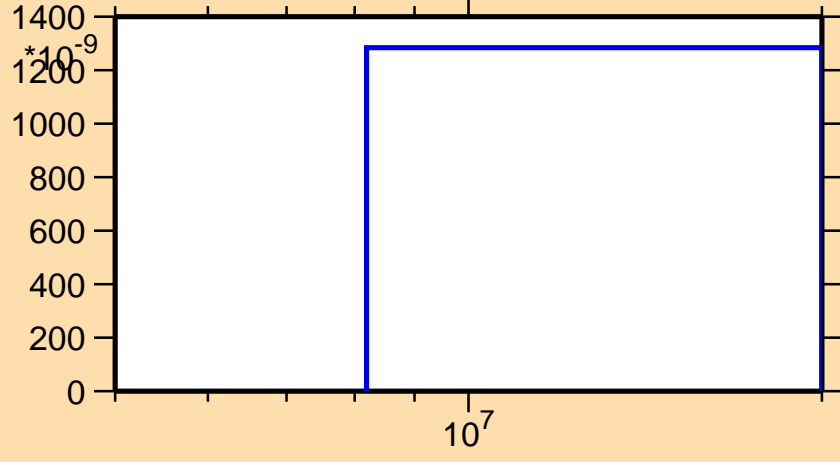
\sigma vs. E for ^{176}\text{Ta}(n,2n\alpha)
