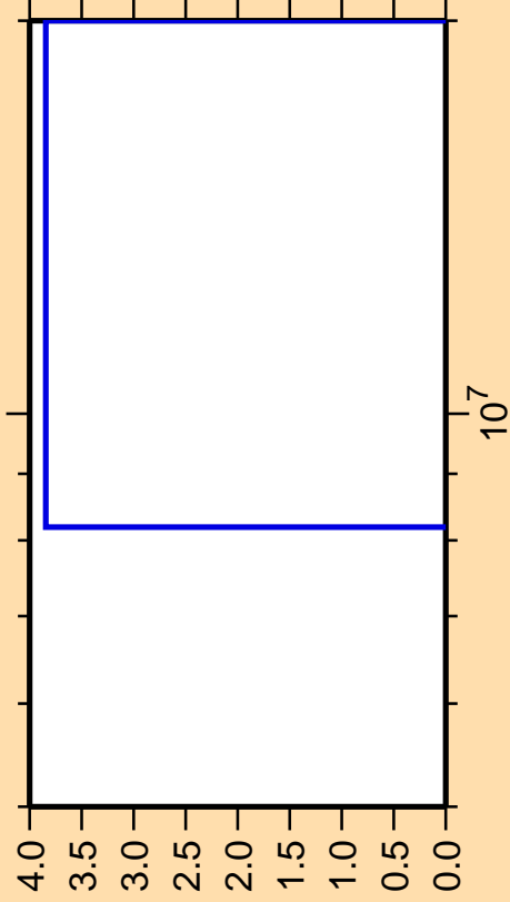
\Delta\sigma/\sigma vs. E for ^{176}\text{Ta} (mt 45)
