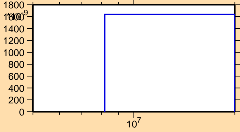
\sigma vs. E for ^{176}\text{Ta}(n,\text{nd})
