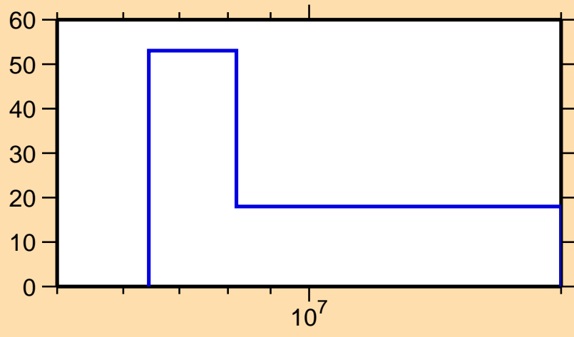
\Delta\sigma/\sigma vs. E for ^{176}\text{Ta}(n,2n)
