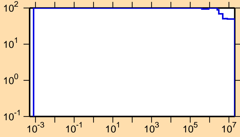
\Delta\sigma/\sigma vs. E for ^{176}\text{Ta}(n,p)
