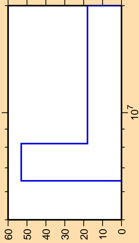
\Delta\sigma/\sigma vs. E for ^{176}\text{Ta}(n,2n)
