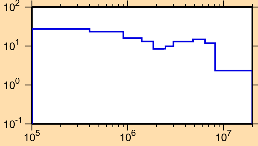
\Delta\sigma/\sigma vs. E for ^{176}\text{Ta}(n,\text{tot.})
