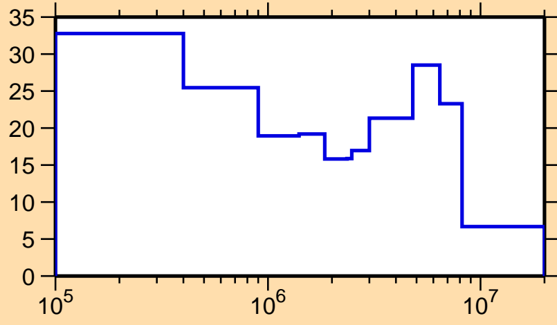
\Delta\sigma/\sigma vs. E for ^{176}\text{Ta}(n,\text{el.})
