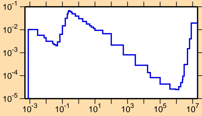
\sigma vs. E for ^{176}\text{Ta}(n,p)
