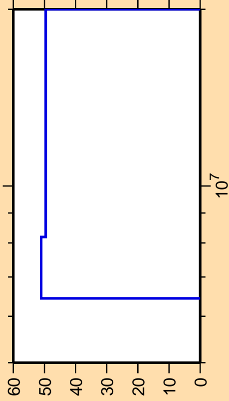
\Delta\sigma/\sigma vs. E for ^{176}\text{Ta}(n,p)
