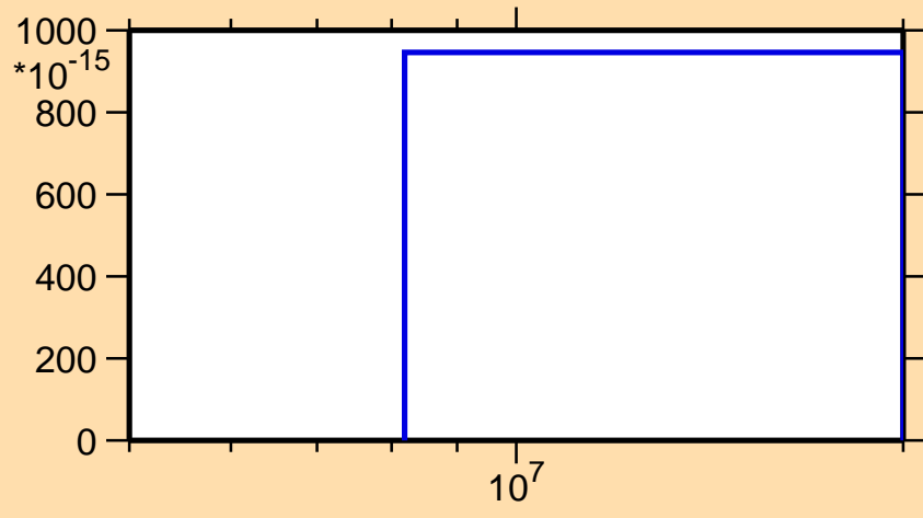
\sigma vs. E for ^{176}\text{Ta}(\text{mt117})
