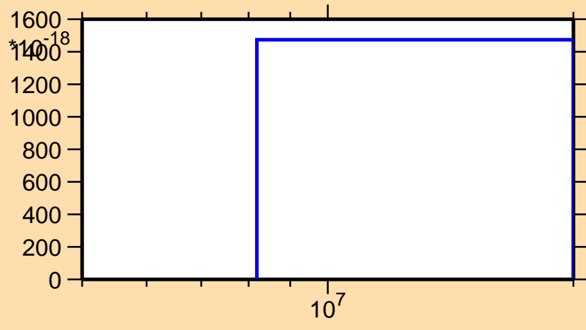
\sigma vs. E for ^{176}\text{Ta}(n,\text{pt})
