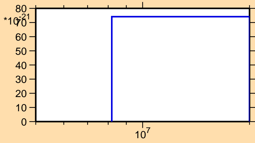
\sigma vs. E for ^{177}\text{Ta} (mt 42)
