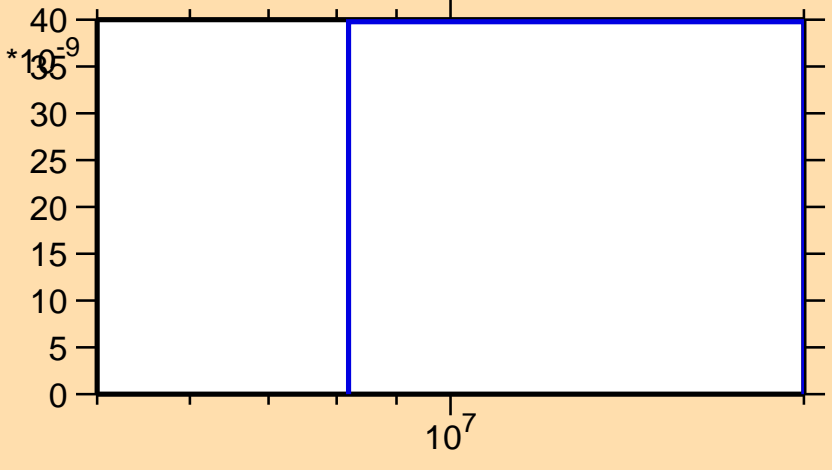
\sigma vs. E for ^{177}\text{Ta}(n,2n\alpha)
