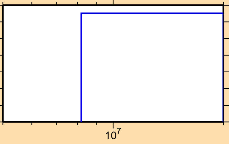
\sigma vs. E for ^{178}\text{Ta}(n,\text{He}3)
