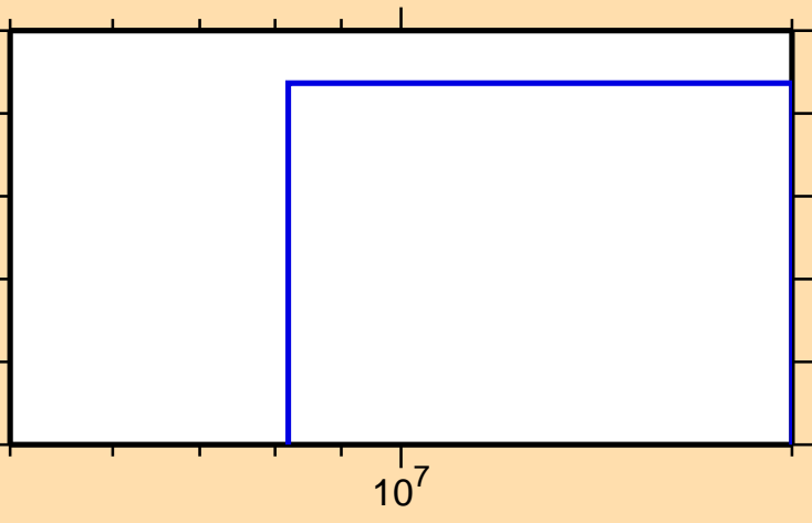
\sigma vs. E for ^{178}\text{Ta}(n,3n\alpha)
