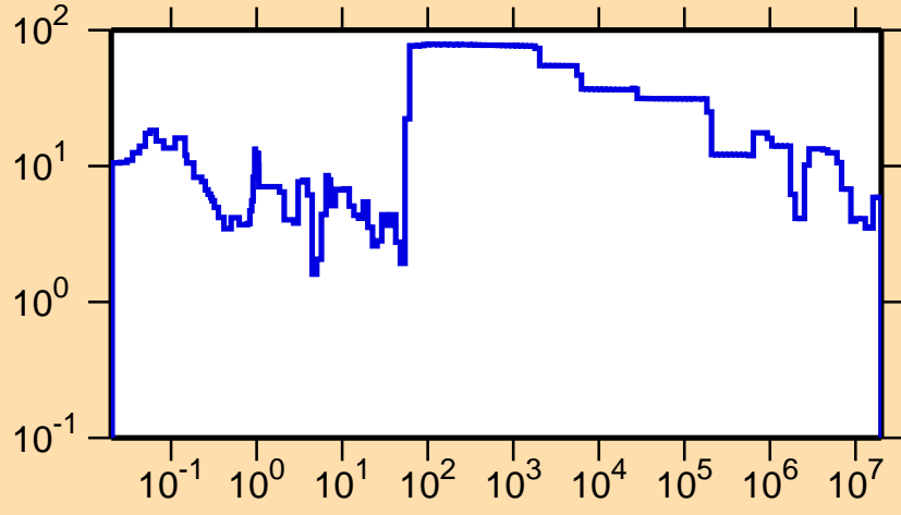
\Delta\sigma/\sigma vs. E for ^{179}\text{Ta}(n,\text{tot.})
