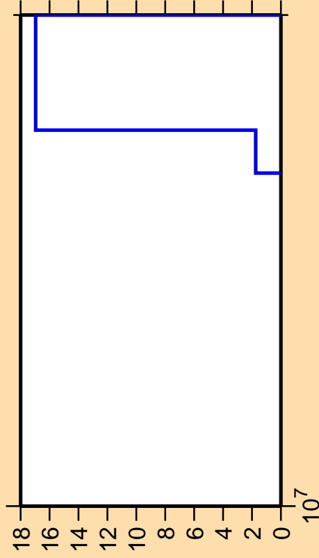
\Delta\sigma/\sigma vs. E for ^{179}\text{Ta}(\text{mt117})
