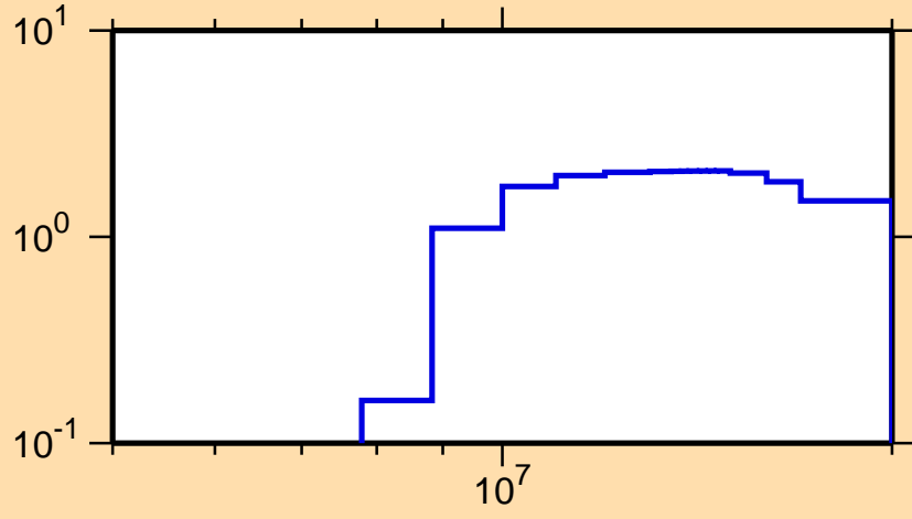
\sigma vs. E for ^{179}\text{Ta}(n,2n)
