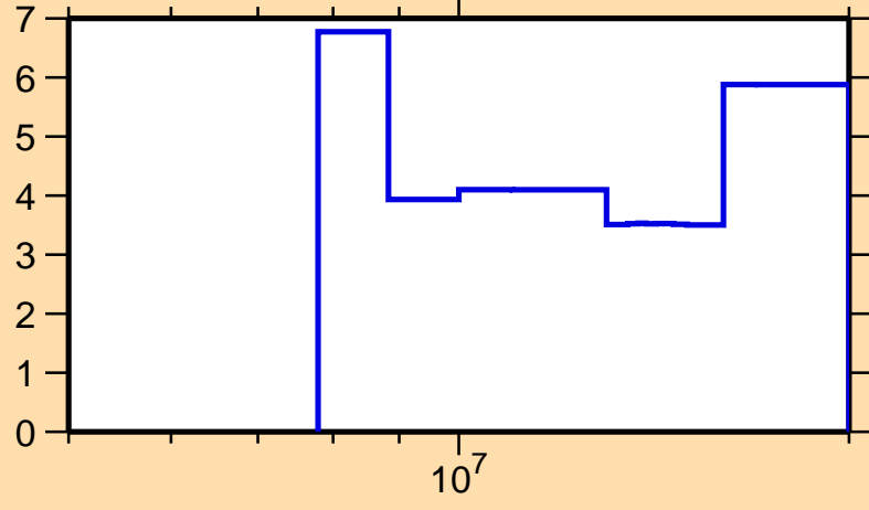
\Delta\sigma/\sigma vs. E for ^{179}\text{Ta}(n,\text{tot.})
