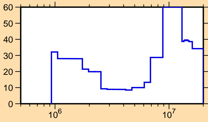
\Delta\sigma/\sigma vs. E for ^{179}\text{Ta}(n,\text{inel.})
