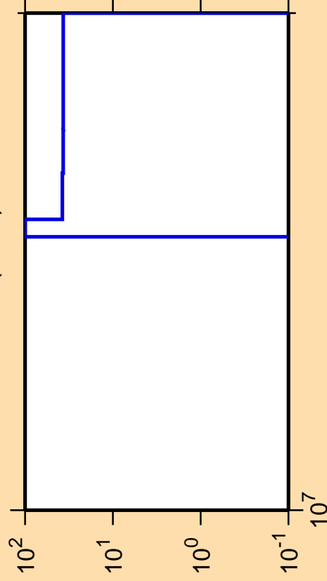
\Delta\sigma/\sigma vs. E for ^{179}\text{Ta}(n,3n)
