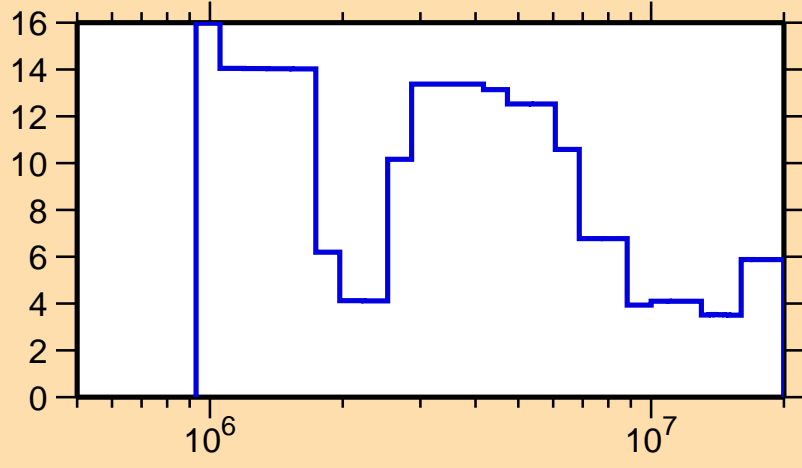
\Delta\sigma/\sigma vs. E for ^{179}\text{Ta}(n,\text{tot.})
