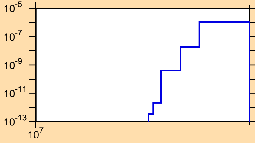
\sigma vs. E for ^{179}\text{Ta}(n,nt)
