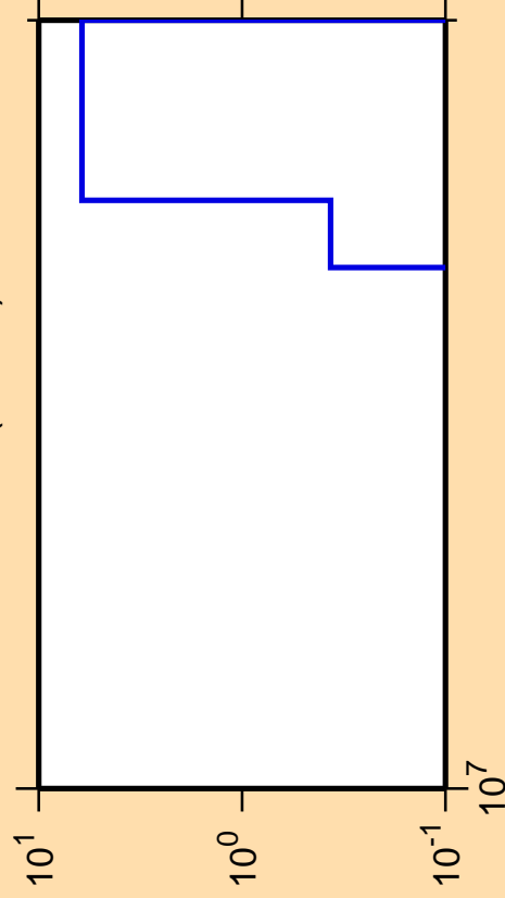
\Delta\sigma/\sigma vs. E for ^{179}\text{Ta} (mt 45)
