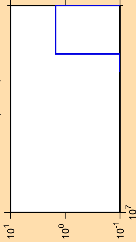
\Delta\sigma/\sigma vs. E for ^{179}\text{Ta}(n,3n\alpha)
