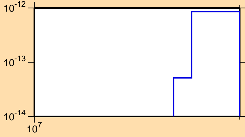
\sigma vs. E for ^{179}\text{Ta} (mt 45)
