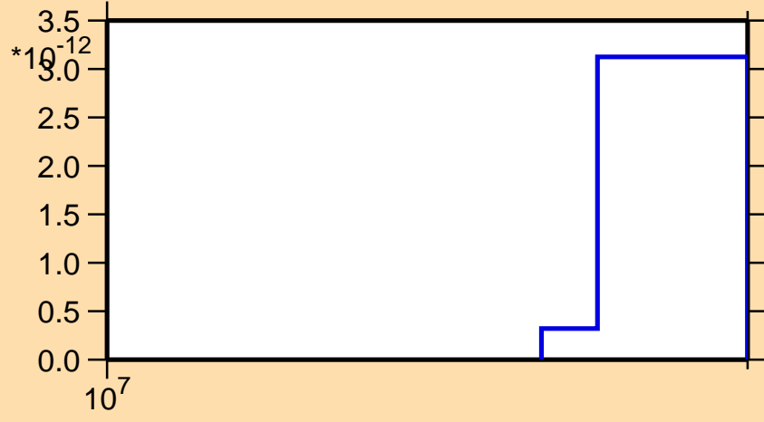
\sigma vs. E for ^{179}\text{Ta}(\text{mt117})
