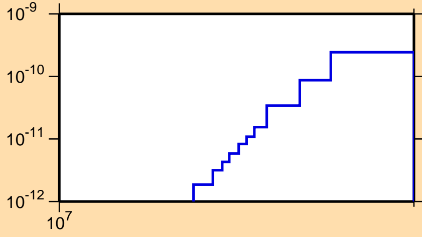
\sigma vs. E for ^{179}\text{Ta}(n,p\alpha)
