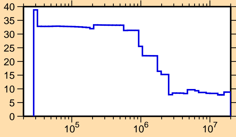
\Delta\sigma/\sigma vs. E for ^{179}\text{Ta}(n,\text{nonel.})
