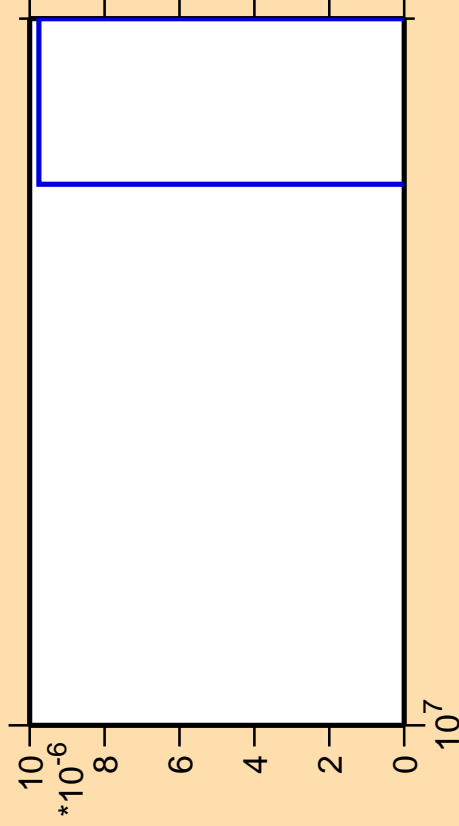
\Delta\sigma/\sigma vs. E for ^{179}\text{Ta} (mt 42)
