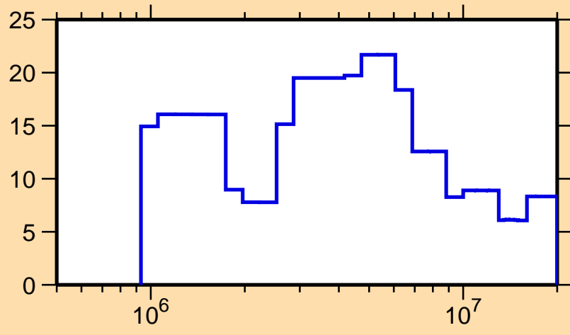
\Delta\sigma/\sigma vs. E for ^{179}\text{Ta}(n,\text{el.})
