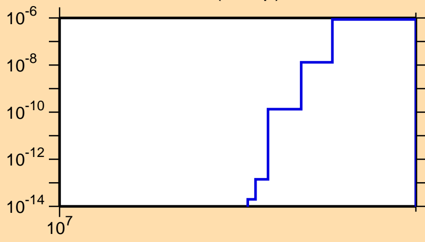
\sigma vs. E for ^{179}\text{Ta}(n,2np)
