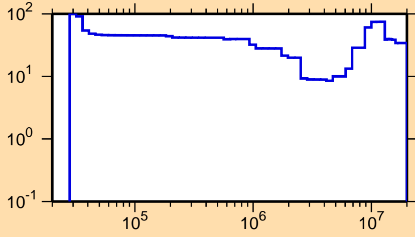
\Delta\sigma/\sigma vs. E for ^{179}\text{Ta}(n,\text{inel.})
