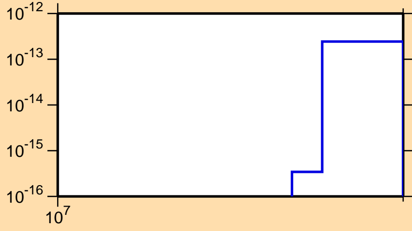
\sigma vs. E for ^{179}\text{Ta}(n,3n\alpha)
