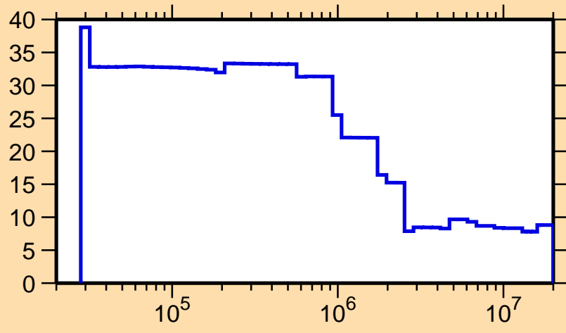
\Delta\sigma/\sigma vs. E for ^{179}\text{Ta}(n,\text{nonel.})
