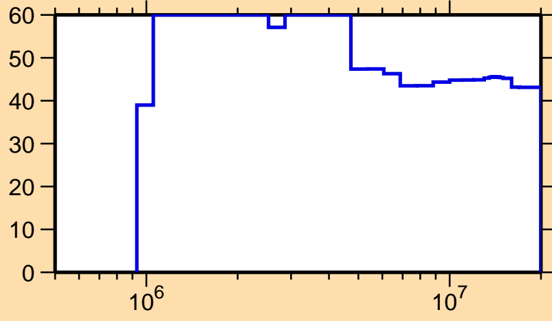
\Delta\sigma/\sigma vs. E for ^{179}\text{Ta}(n,n_1)
