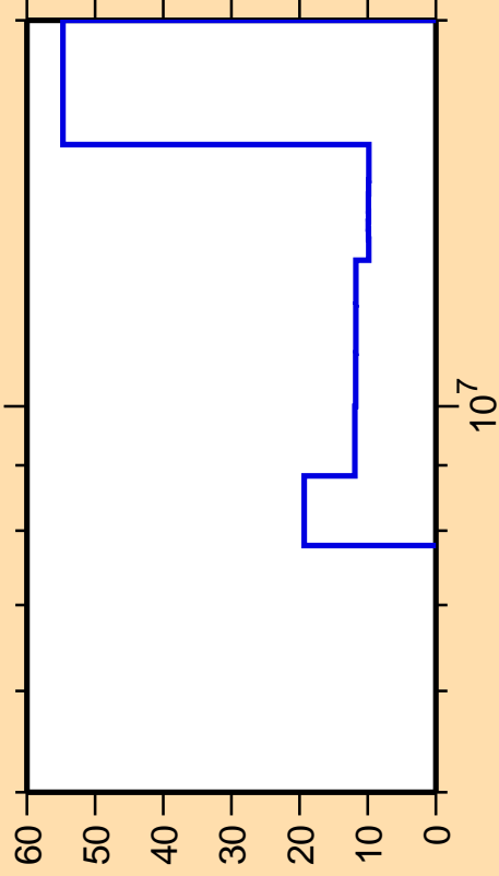
\Delta\sigma/\sigma vs. E for ^{179}\text{Ta}(n,2n)
