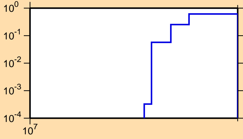
\sigma vs. E for ^{179}\text{Ta}(n,3n)
