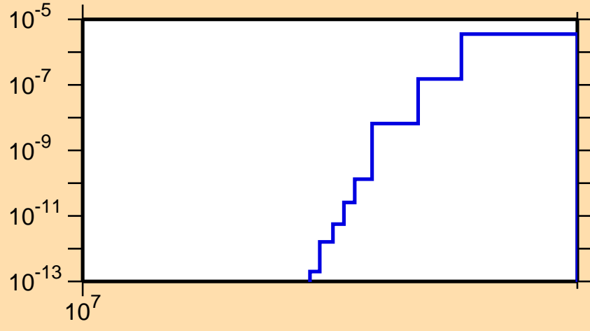
\sigma vs. E for ^{179}\text{Ta}(n,\text{nd})
