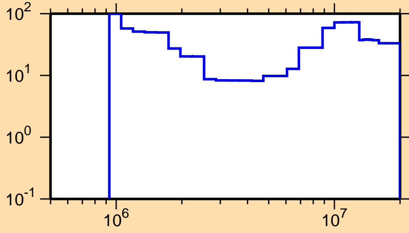
\Delta\sigma/\sigma vs. E for ^{179}\text{Ta}(n,n\text{cont.})
