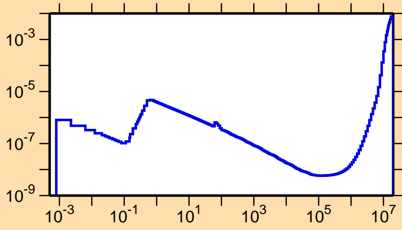
\sigma vs. E for ^{179}\text{Ta}(n,\alpha)
