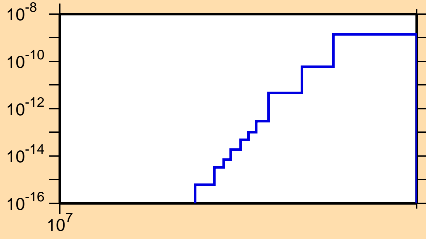
\sigma vs. E for ^{179}\text{Ta}(n,\text{He3})
