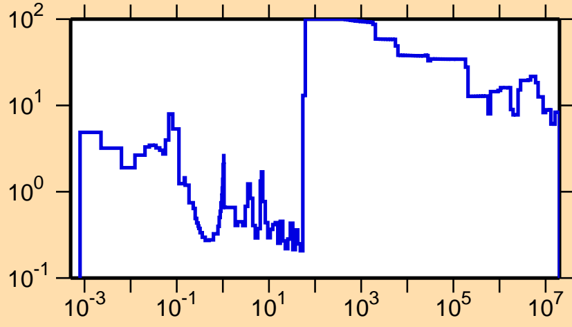
\Delta\sigma/\sigma vs. E for ^{179}\text{Ta}(n,\text{el.})
