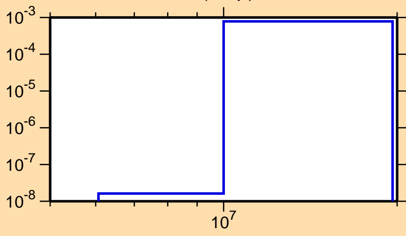
\sigma vs. E for ^{179}\text{Ta}(n,np)
