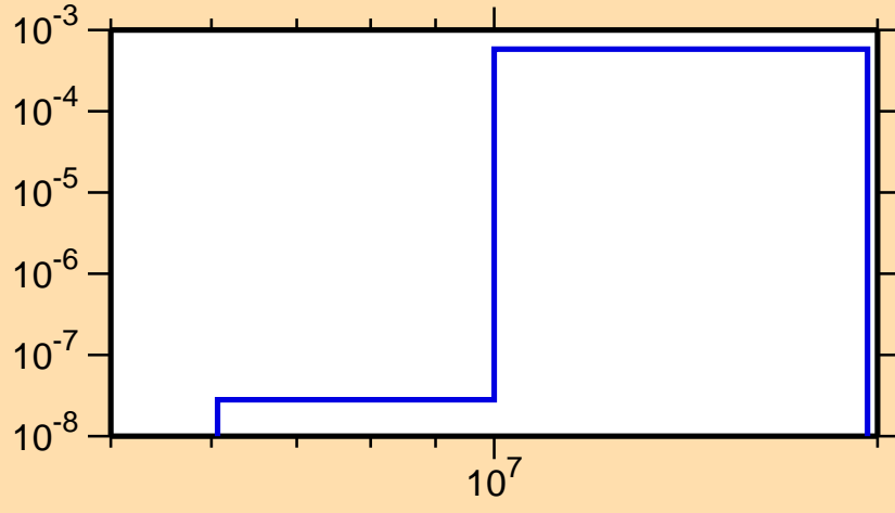
\sigma vs. E for ^{179}\text{Ta}(n,d)
