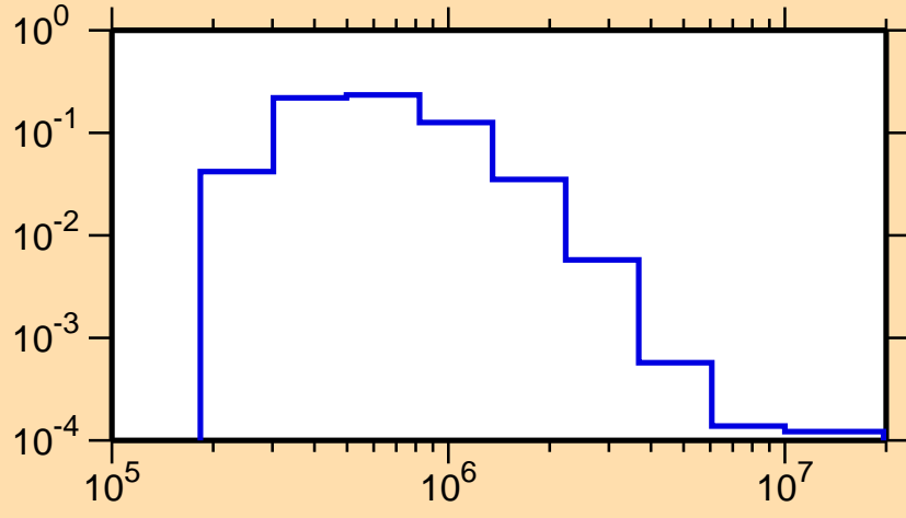
\sigma vs. E for ^{179}\text{Ta}(n,n_4)
