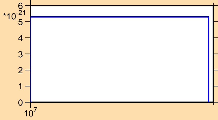
\sigma vs. E for ^{179}\text{Ta} (mt 42)
