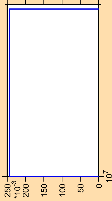
\Delta\sigma/\sigma vs. E for ^{179}\text{Ta}(\text{mt117})
