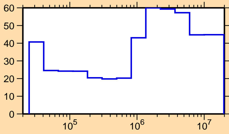
\Delta\sigma/\sigma vs. E for ^{179}\text{Ta}(n,n_1)
