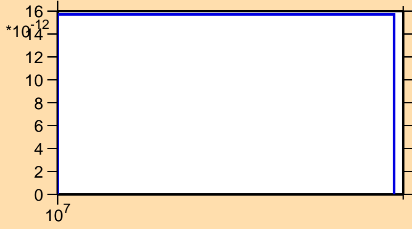
\sigma vs. E for ^{179}\text{Ta}(n,p\alpha)
