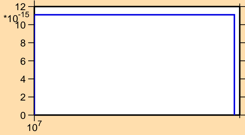
\sigma vs. E for ^{179}\text{Ta} (mt 45)
