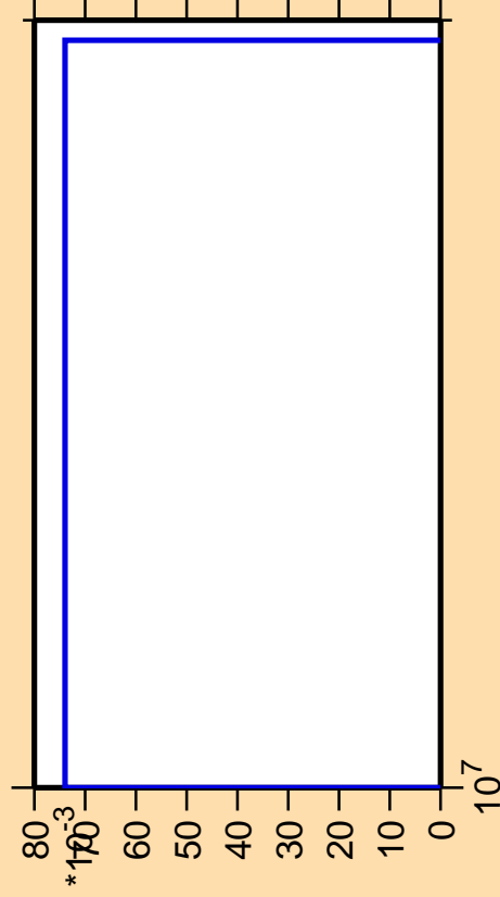
\Delta\sigma/\sigma vs. E for ^{179}\text{Ta} (mt 45)
