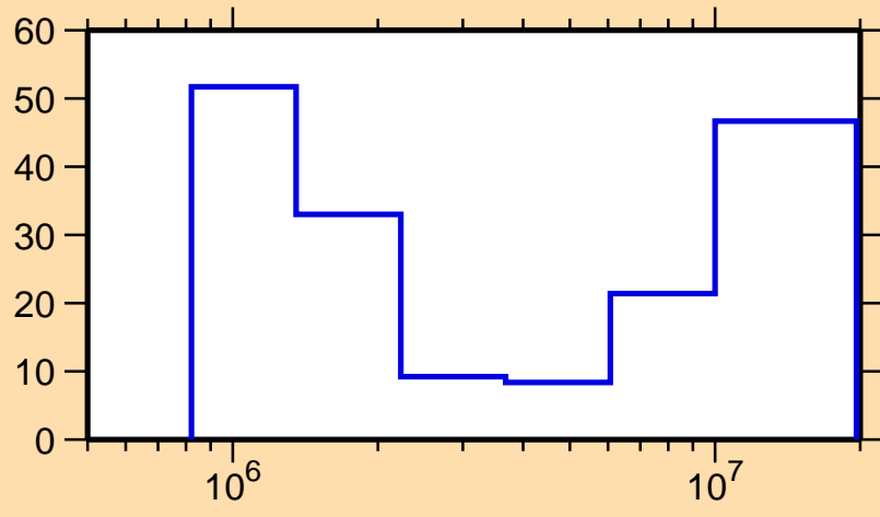
\Delta\sigma/\sigma vs. E for ^{179}\text{Ta}(n,n\text{cont.})
