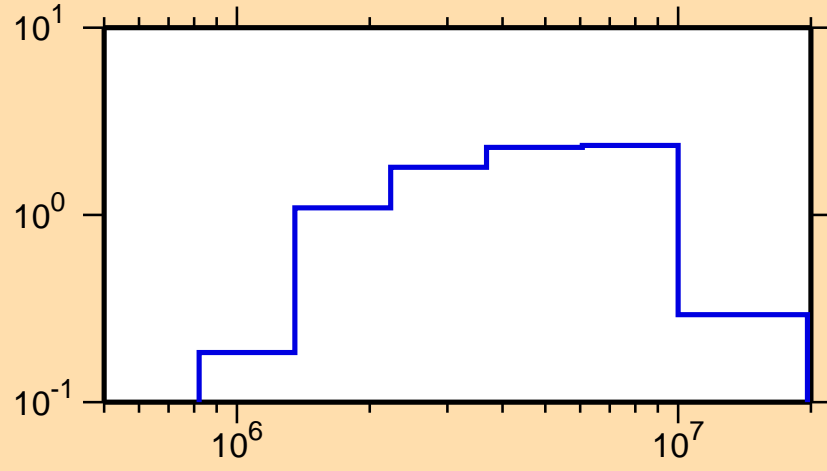
\sigma vs. E for ^{179}\text{Ta}(n,n\text{cont.})
