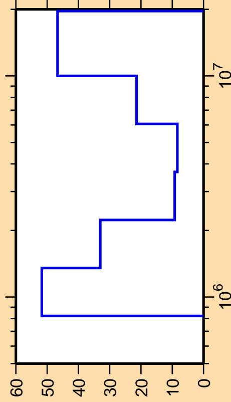
\Delta\sigma/\sigma vs. E for ^{179}\text{Ta}(n,n\text{cont.})
