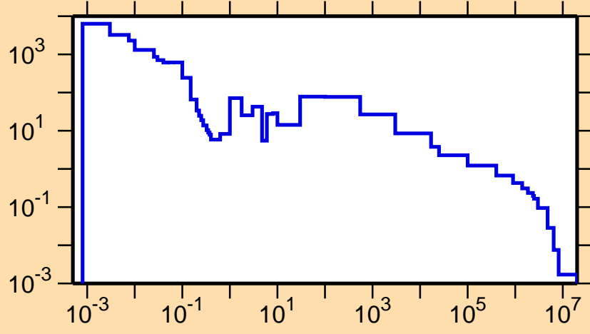
\sigma vs. E for ^{179}\text{Ta}(n,\gamma)
