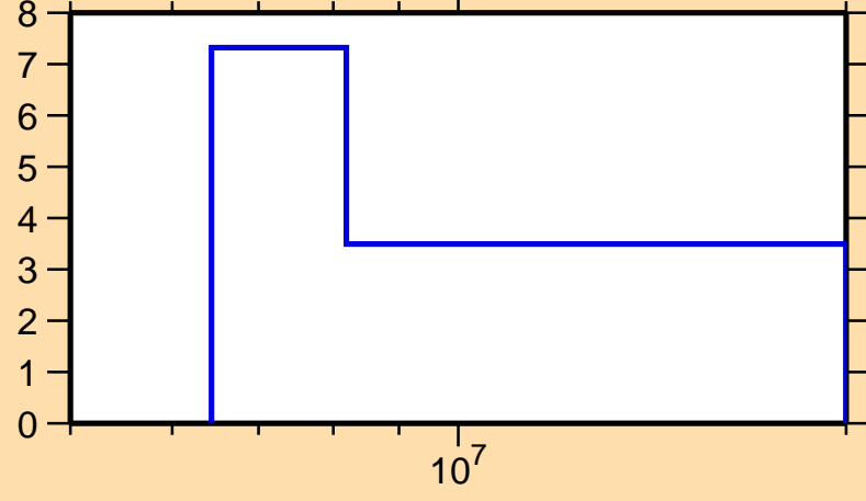
\Delta\sigma/\sigma vs. E for ^{179}\text{Ta}(n,\text{tot.})
