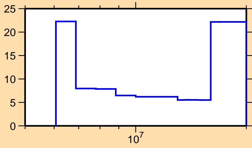
\Delta\sigma/\sigma vs. E for ^{180}\text{Ta}(n,2n)
