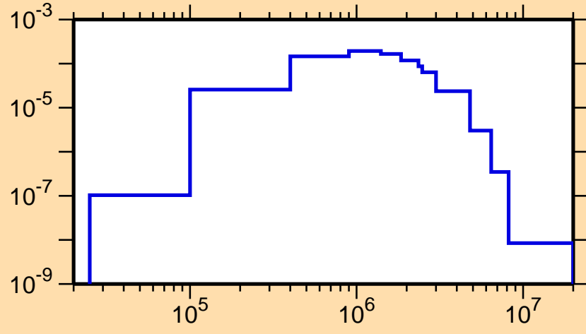
\sigma vs. E for ^{180}\text{Ta}(n,n_4)
