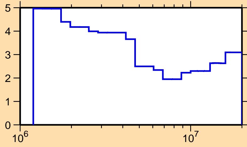
\Delta\sigma/\sigma vs. E for ^{181}\text{Ta}(n,\text{tot.})
