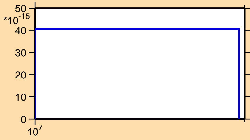
\sigma vs. E for ^{181}\text{Ta}(n,p\alpha)
