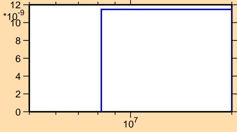
\sigma vs. E for ^{181}\text{Ta}(n,\text{nd})
