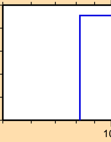
\sigma vs. E for ^{181}\text{Ta}(n,\text{He3})
