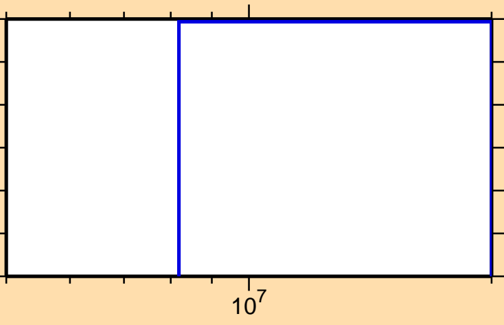
\sigma vs. E for ^{181}\text{Ta}(n,nt)
