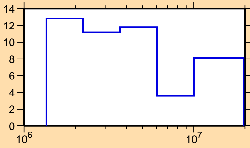
\Delta\sigma/\sigma vs. E for ^{182}\text{Ta}(n,el.)
