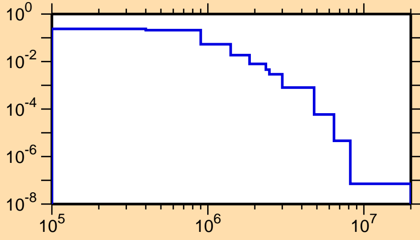
\sigma vs. E for ^{182}\text{Ta}(n,n_3)
