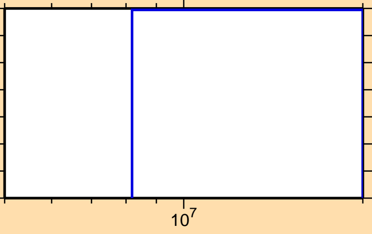
\sigma vs. E for ^{182}\text{Ta}(n,nt)
