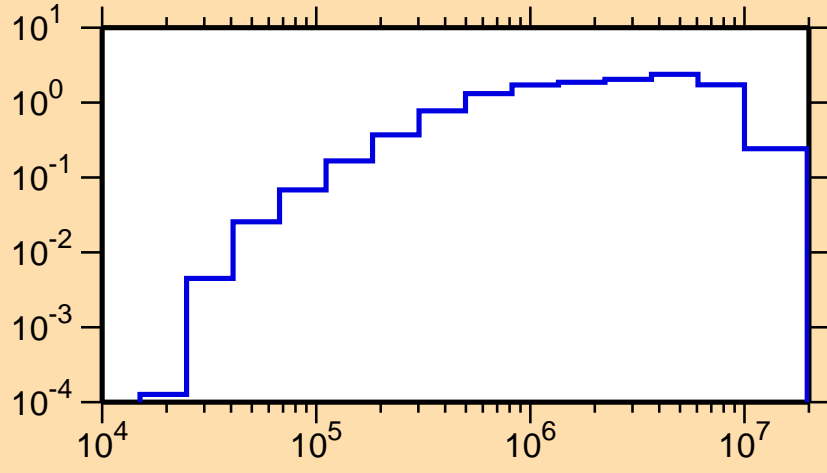
\sigma vs. E for ^{182}\text{Ta}(n,n\text{cont.})
