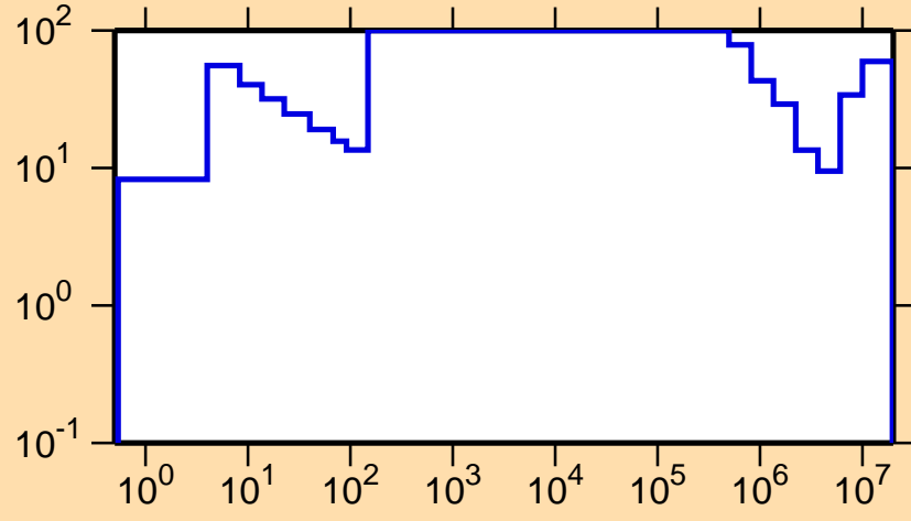
\Delta\sigma/\sigma vs. E for ^{182}\text{Ta}(n,n\text{cont.})
