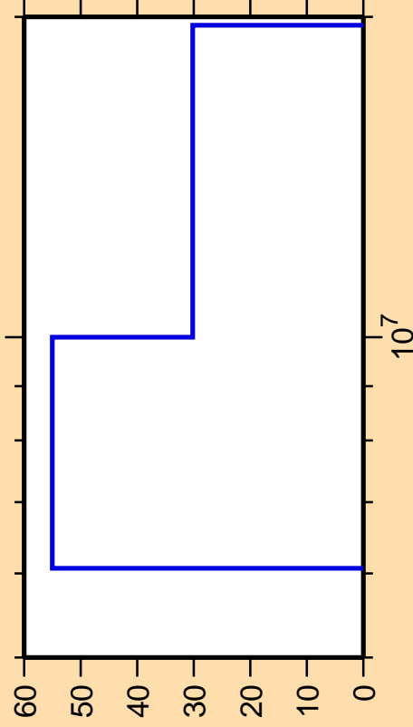
\Delta\sigma/\sigma vs. E for ^{182}\text{Ta}(n,np)
