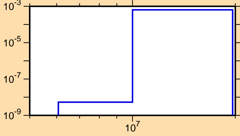
\sigma vs. E for ^{182}\text{Ta}(n,d)
