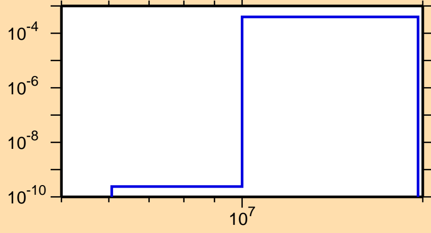
\sigma vs. E for ^{182}\text{Ta}(n,np)
