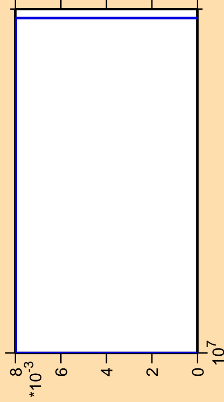
\Delta\sigma/\sigma vs. E for ^{182}\text{Ta}(n,3n\alpha)
