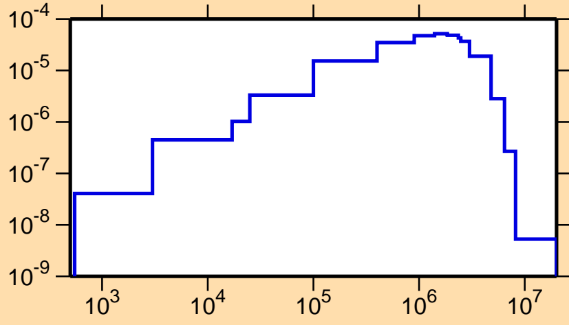
\sigma vs. E for ^{182}\text{Ta}(n,n_1)
