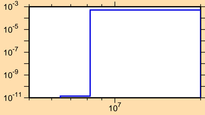
\sigma vs. E for ^{182}\text{Ta}(n,d)
