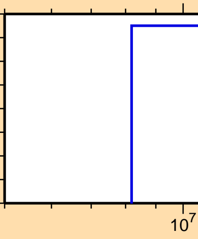
\sigma vs. E for ^{182}\text{Ta}(n,np)
