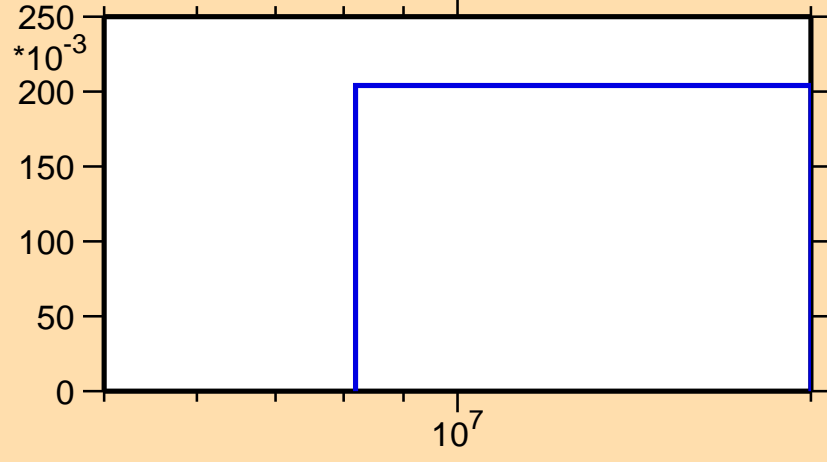
\sigma vs. E for ^{183}\text{Ta}(n,3n)
