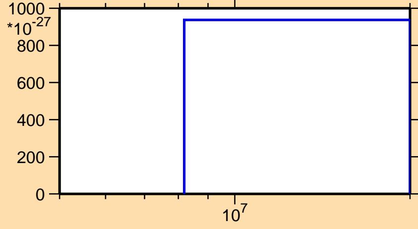
\sigma vs. E for ^{183}\text{Ta} (mt 42)
