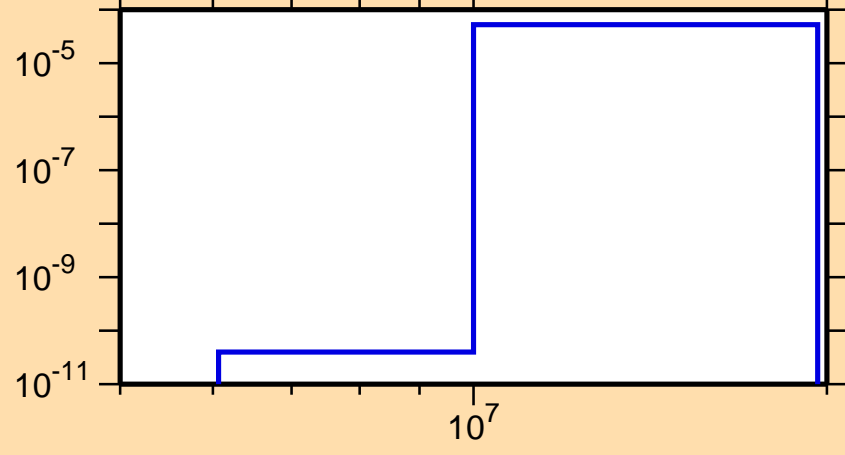
\sigma vs. E for ^{184}\text{Ta}(n,t)
