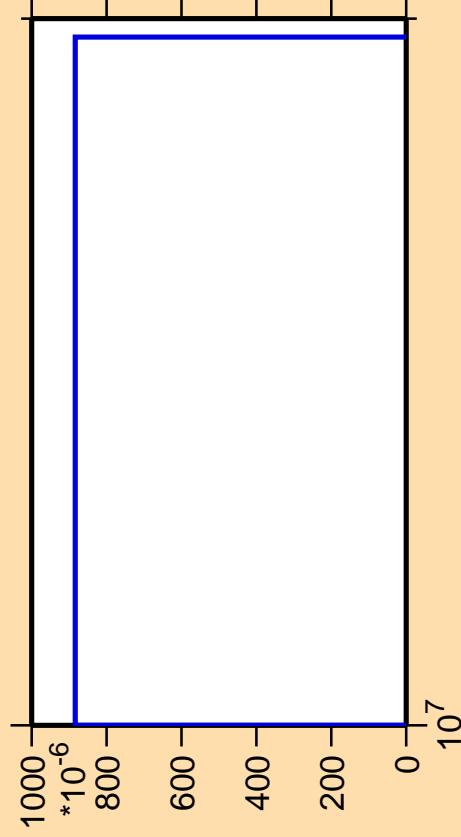
\Delta\sigma/\sigma vs. E for ^{184}\text{Ta}(n,3n\alpha)
