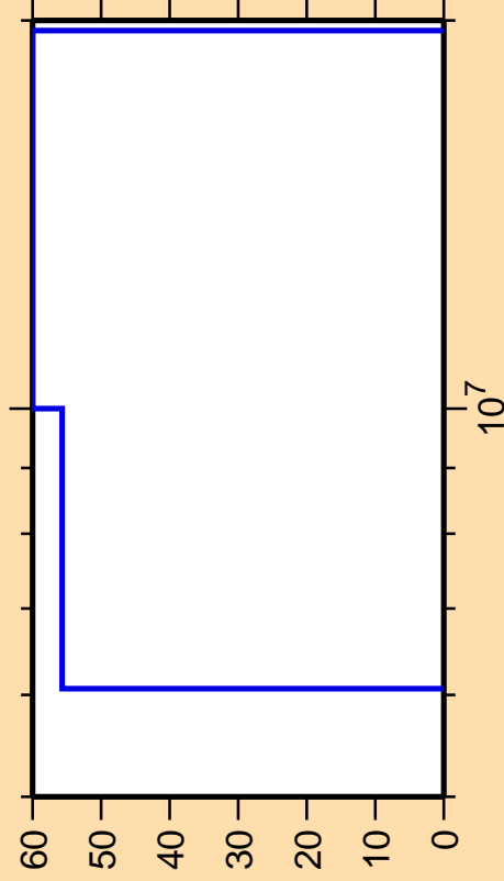
\Delta\sigma/\sigma vs. E for ^{184}\text{Ta}(n,t)
