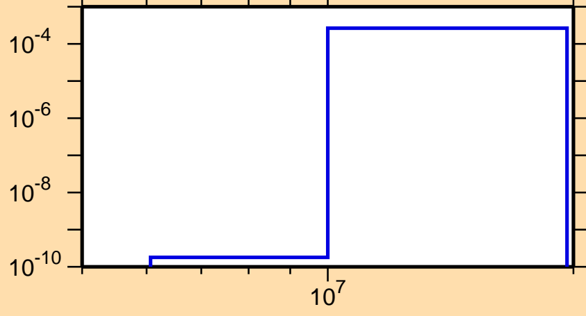
\sigma vs. E for ^{184}\text{Ta}(n,d)
