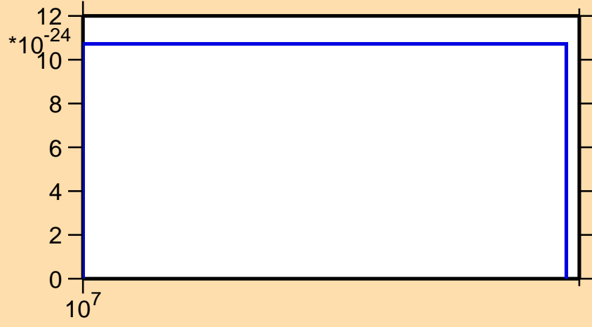
\sigma vs. E for ^{184}\text{Ta} (mt 42)
