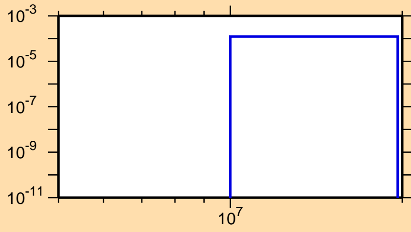
\sigma vs. E for ^{184}\text{Ta}(n,np)
