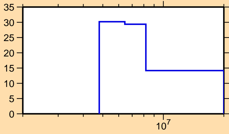
\Delta\sigma/\sigma vs. E for ^{184}\text{Ta}(n,2n)
