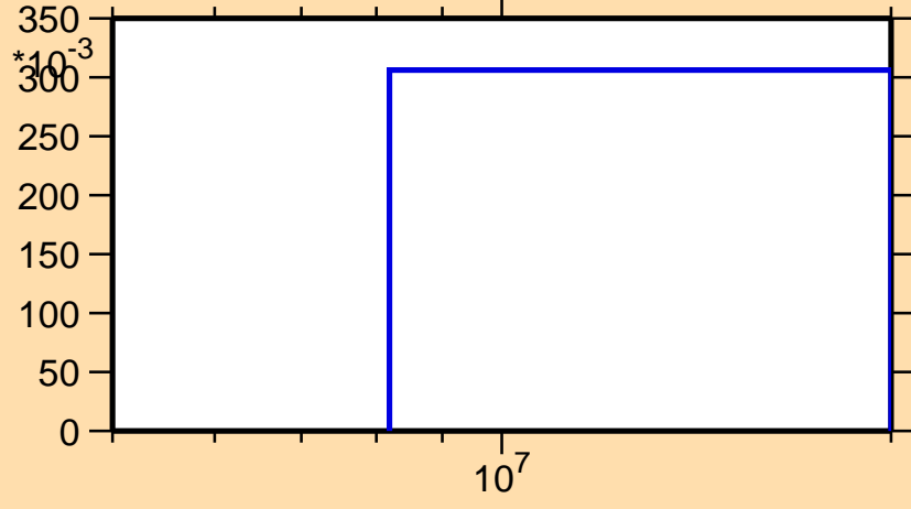
\sigma vs. E for ^{184}\text{Ta}(n,3n)
