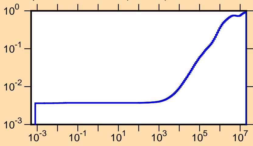
\mu vs. E for ^{185}\text{Ta}(\text{mt251})
