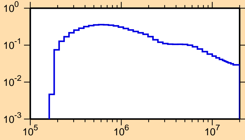
\sigma vs. E for ^{185}\text{Ta}(n,n_2)
