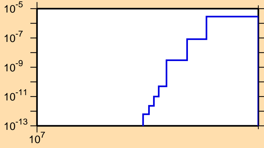
\sigma vs. E for ^{185}\text{Ta}(n,nt)
