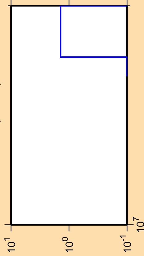
\Delta\sigma/\sigma vs. E for ^{185}\text{Ta}(n,\text{He3})
