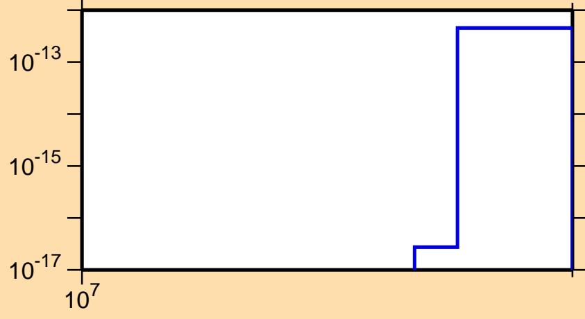
\sigma vs. E for ^{185}\text{Ta}(n,3n\alpha)
