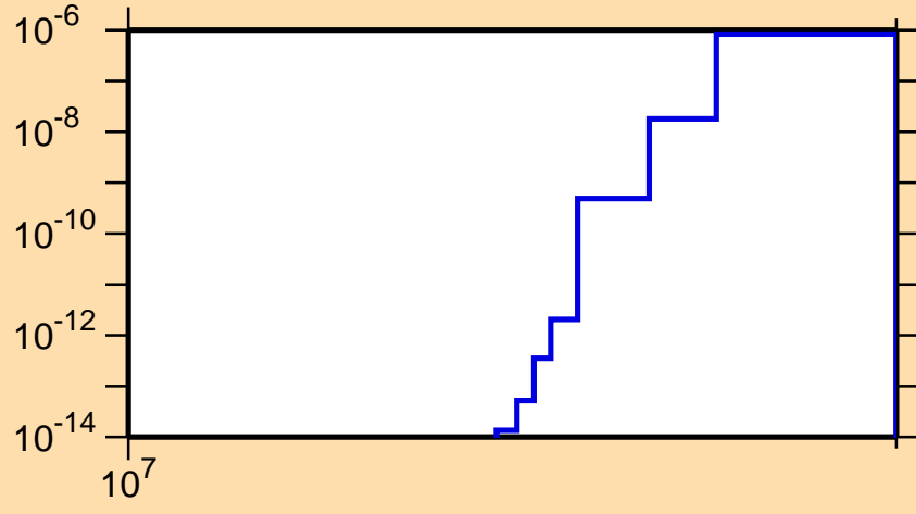
\sigma vs. E for ^{185}\text{Ta}(n,\text{nd})
