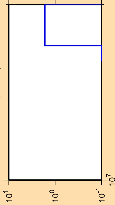
\Delta\sigma/\sigma vs. E for ^{185}\text{Ta}(n,3n\alpha)
