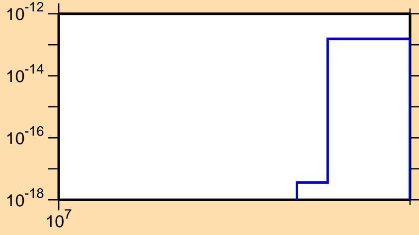
\sigma vs. E for ^{185}\text{Ta}(n,\text{He3})
