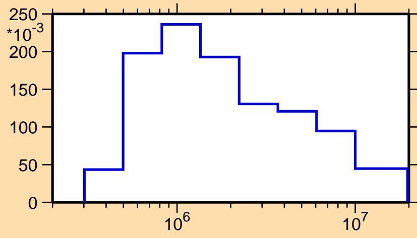
σ vs. E for ^{185}\text{Ta}(n,n_3)
