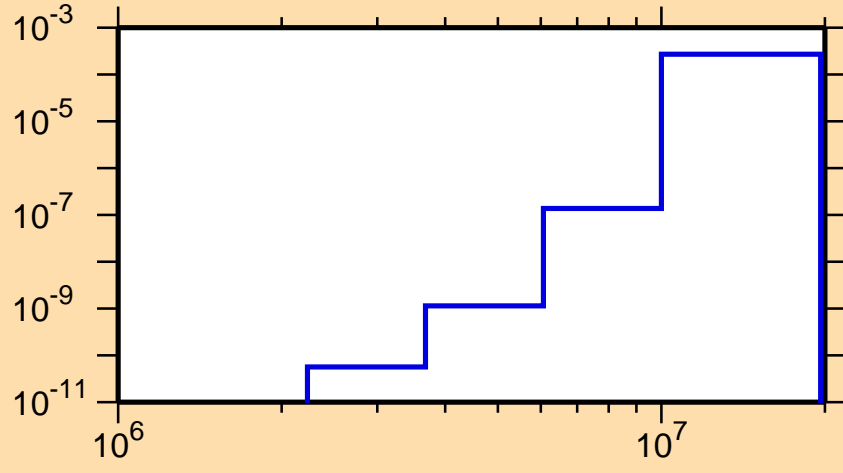
\sigma vs. E for ^{186}\text{Ta}(n,\alpha)
