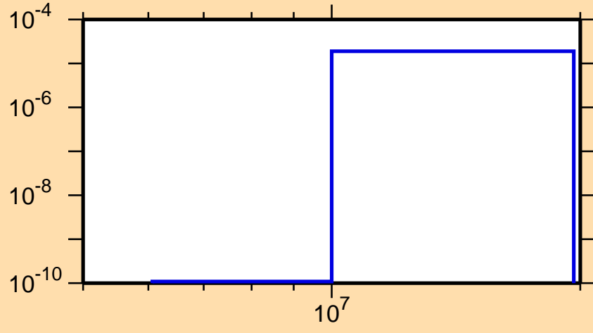
\sigma vs. E for ^{186}\text{Ta}(n,n\alpha)
