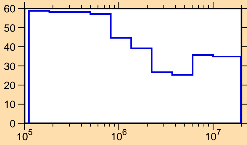
\Delta\sigma/\sigma vs. E for ^{186}\text{Ta}(n,n_1)
