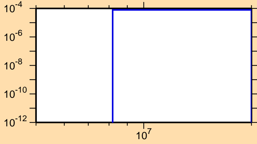
\sigma vs. E for ^{186}\text{Ta}(n,np)
