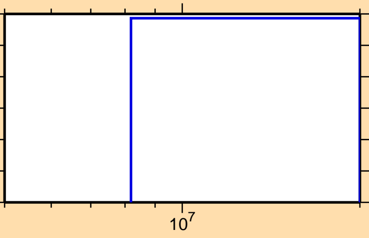
\sigma vs. E for ^{186}\text{Ta}(n,2np)
