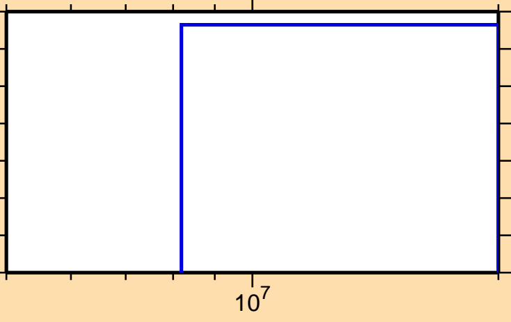
\sigma vs. E for ^{186}\text{Ta}(n,2n\alpha)
