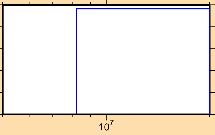
\sigma vs. E for ^{187}\text{Ta}(n,d)
