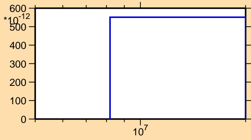
\sigma vs. E for ^{187}\text{Ta}(n,2np)
