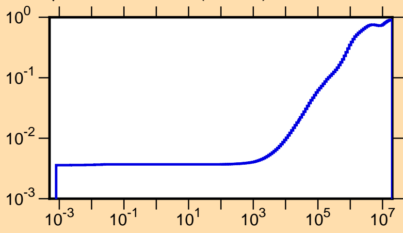
\mu vs. E for ^{188}\text{Ta}(\text{mt251})
