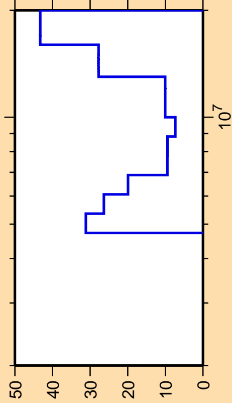
\Delta\sigma/\sigma vs. E for ^{188}\text{Ta}(n,2n)
