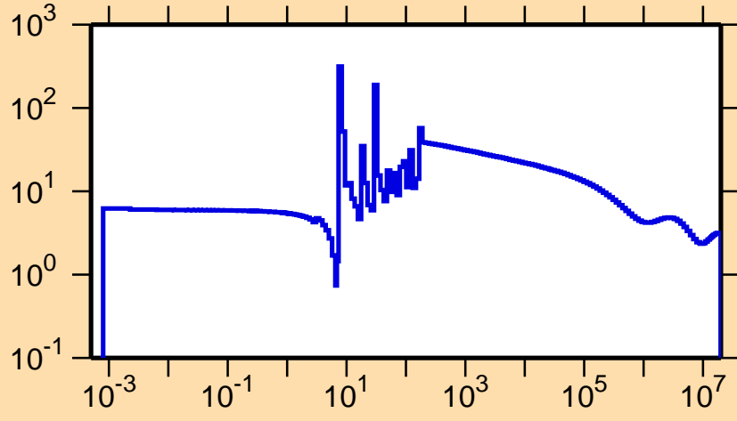
\sigma vs. E for ^{188}\text{Ta}(n,\text{el.})
