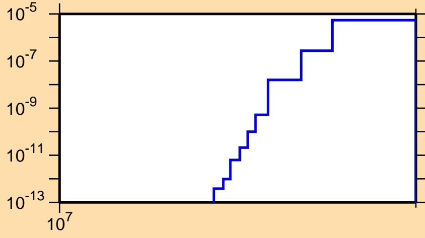
\sigma vs. E for ^{188}\text{Ta}(n,\text{nd})
