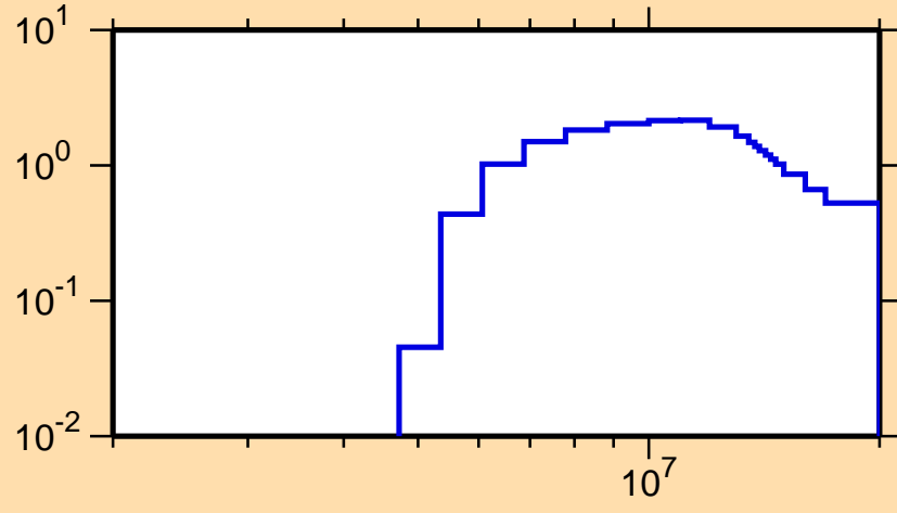
\sigma vs. E for ^{188}\text{Ta}(n,2n)
