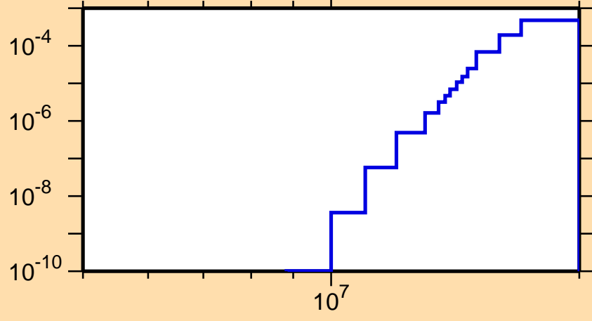
\sigma vs. E for ^{188}\text{Ta}(n,t)
