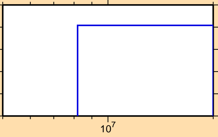
\sigma vs. E for ^{188}\text{Ta}(n,2np)
