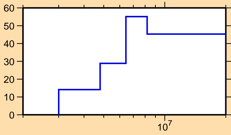
\Delta\sigma/\sigma vs. E for ^{188}\text{Ta}(n,n\text{cont.})
