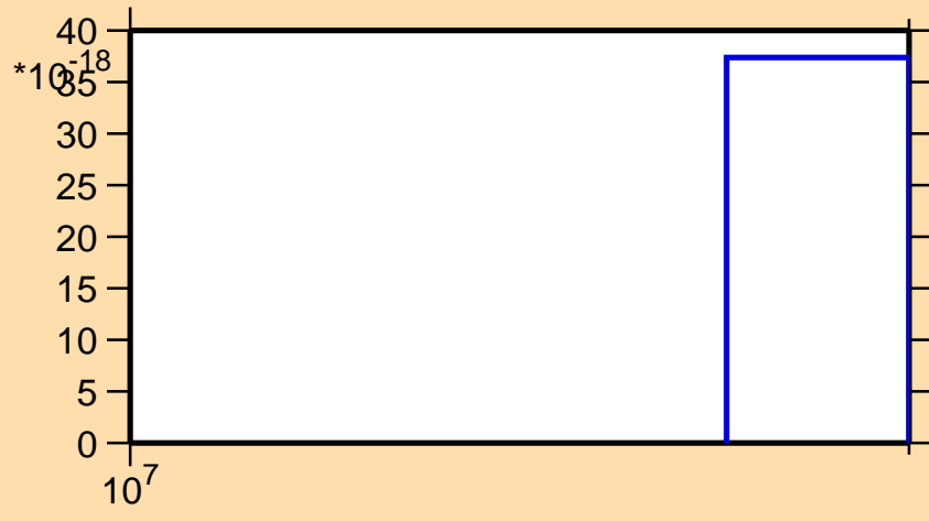
\sigma vs. E for ^{189}\text{Ta} (mt 42)
