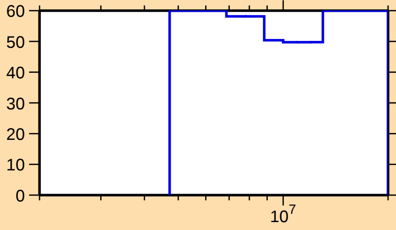
\Delta\sigma/\sigma vs. E for ^{190}\text{Ta}(n,2n)
