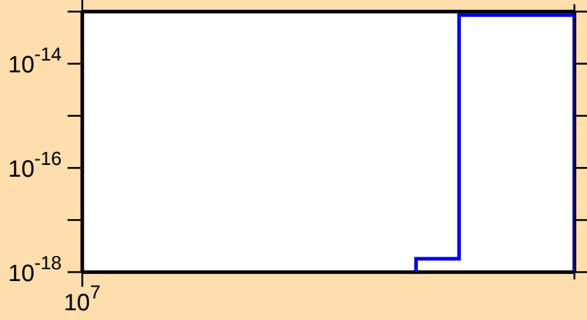
\sigma vs. E for ^{190}\text{Ta}(n,3n\alpha)
