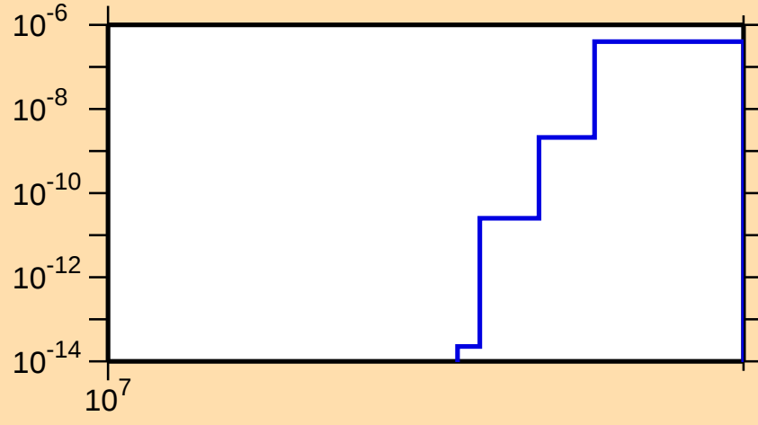
\sigma vs. E for ^{190}\text{Ta}(n,2np)
