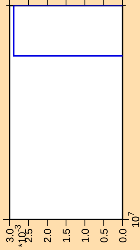
\Delta\sigma/\sigma vs. E for ^{190}\text{Ta}(\text{mt } 42)
