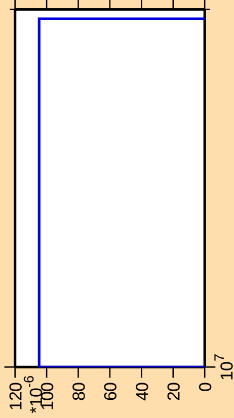
\Delta\sigma/\sigma vs. E for ^{190}\text{Ta}(n,3n\alpha)
