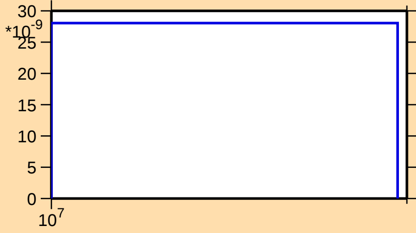
\sigma vs. E for ^{190}\text{Ta}(n,\text{nt})
