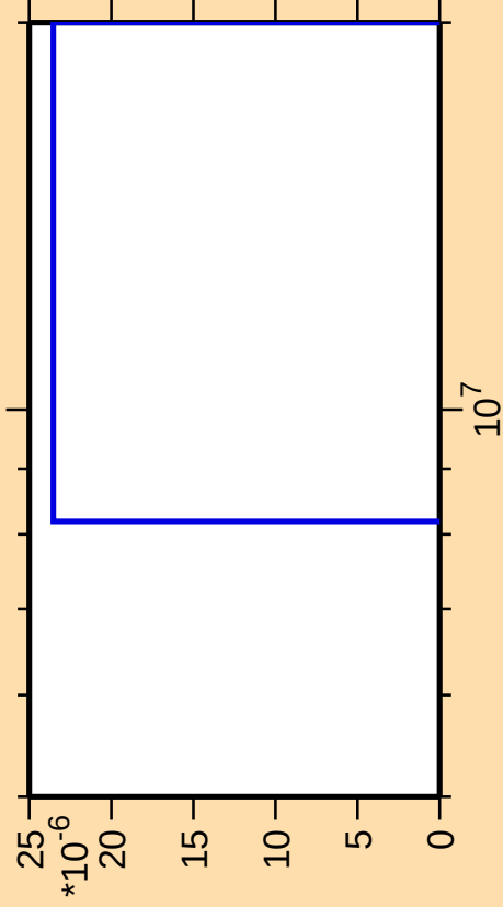
\Delta\sigma/\sigma vs. E for ^{190}\text{Ta}(\text{mt } 42)
