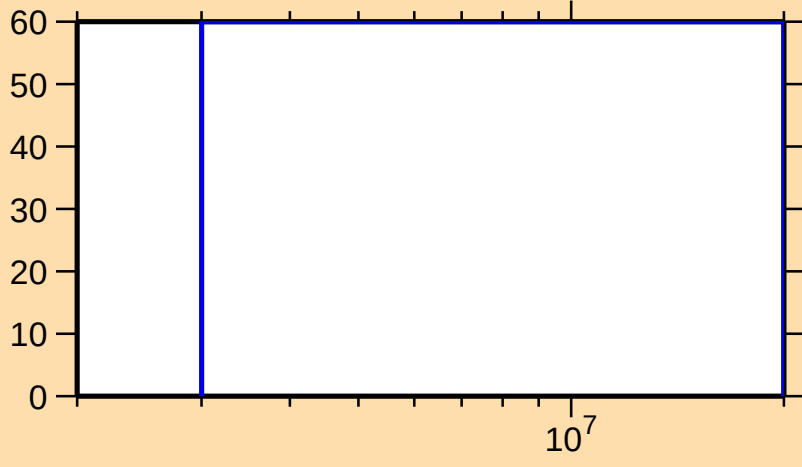
\Delta\sigma/\sigma vs. E for ^{190}\text{Ta}(n,\gamma)
