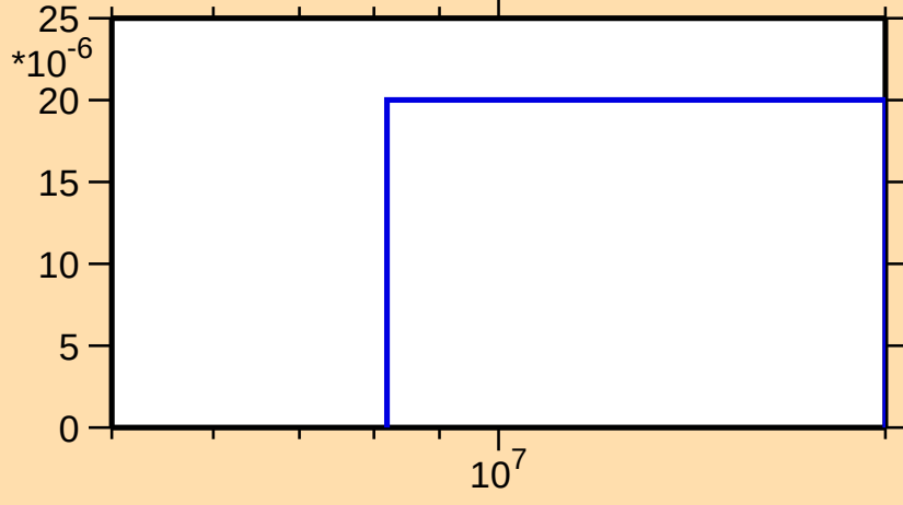
\sigma vs. E for ^{190}\text{Ta}(n,d)
