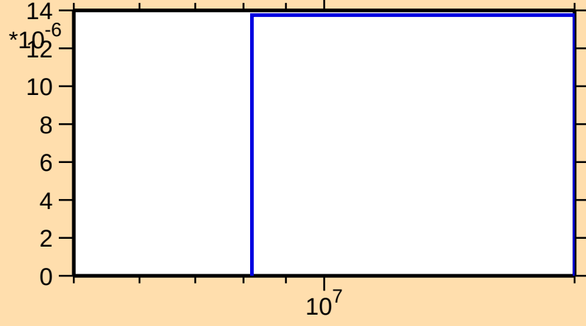
\sigma vs. E for ^{190}\text{Ta}(n,np)
