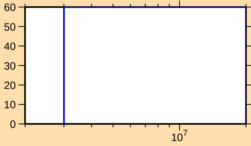
\Delta\sigma/\sigma vs. E for ^{190}\text{Ta}(n,n_1)
