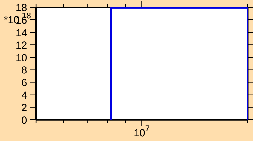
\sigma vs. E for ^{190}\text{Ta}(\text{mt } 42)
