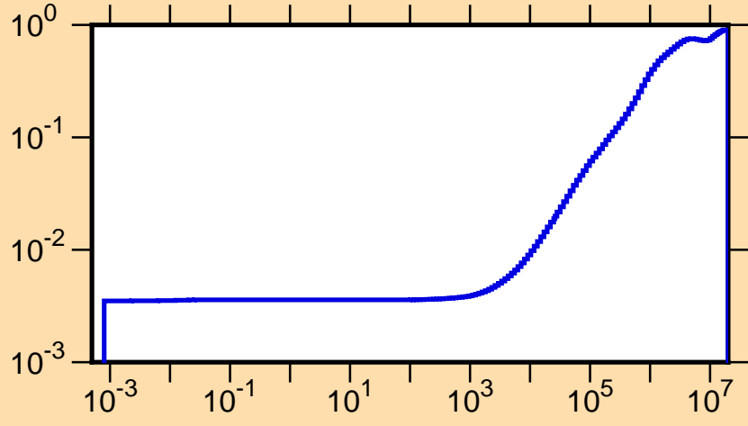
\mu vs. E for ^{192}\text{Ta}(\text{mt251})
