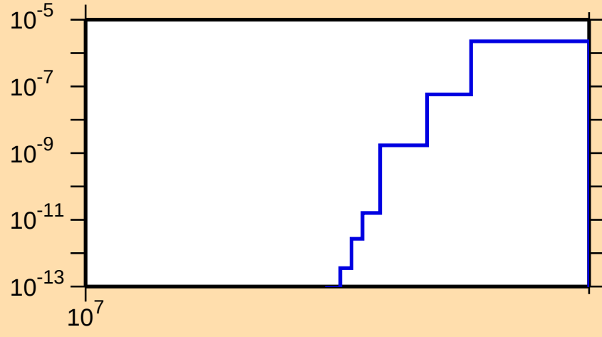
\sigma vs. E for ^{192}\text{Ta}(n,nt)
