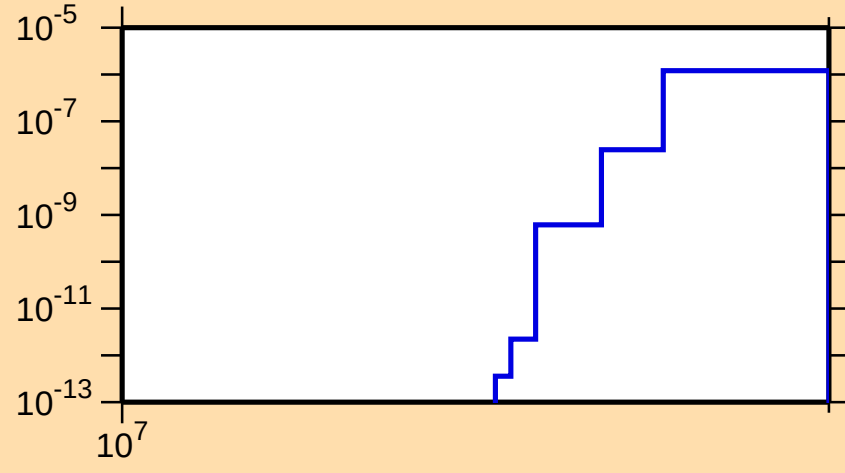
\sigma vs. E for ^{192}\text{Ta}(n,\text{nd})
