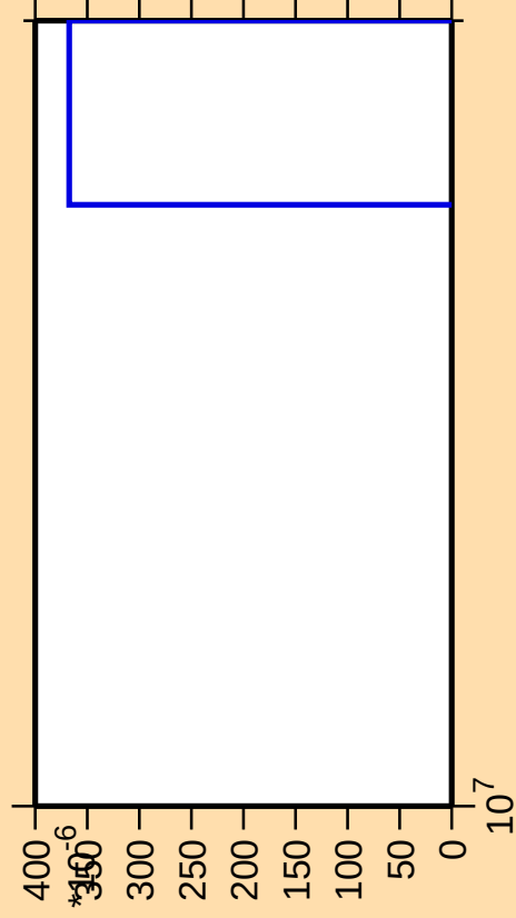
\Delta\sigma/\sigma vs. E for ^{192}\text{Ta}(\text{mt } 42)
