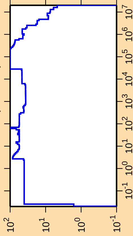
\Delta\sigma/\sigma vs. E for ^{192}\text{Ta}(n,\text{nonel.})
