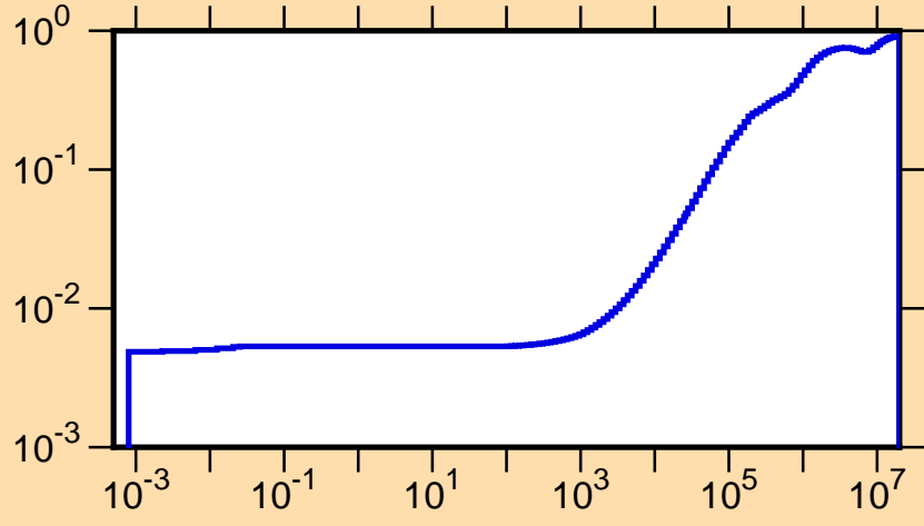
\mu vs. E for ^{139}\text{Tb}(\text{mt251})
