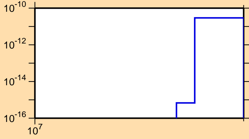
\sigma vs. E for ^{139}\text{Tb}(n,nt)
