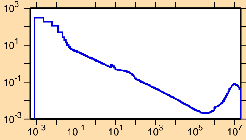
\sigma vs. E for ^{139}\text{Tb}(n,\alpha)
