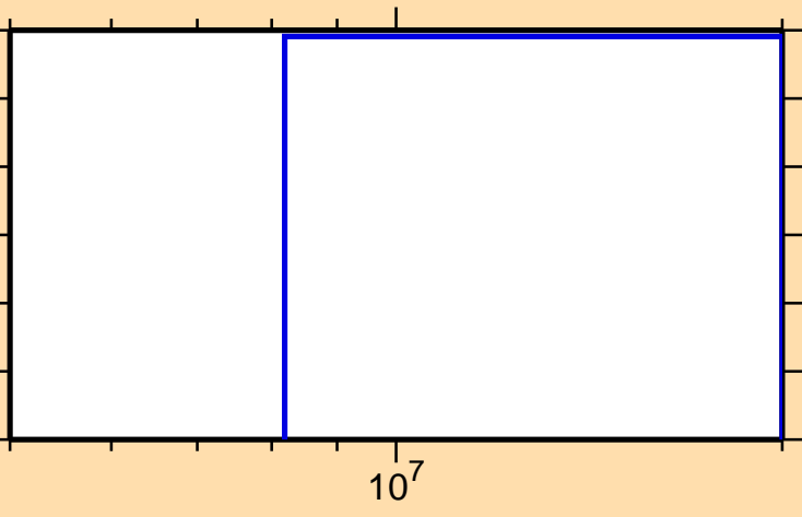
\sigma vs. E for ^{139}\text{Tb}(n,2np)
