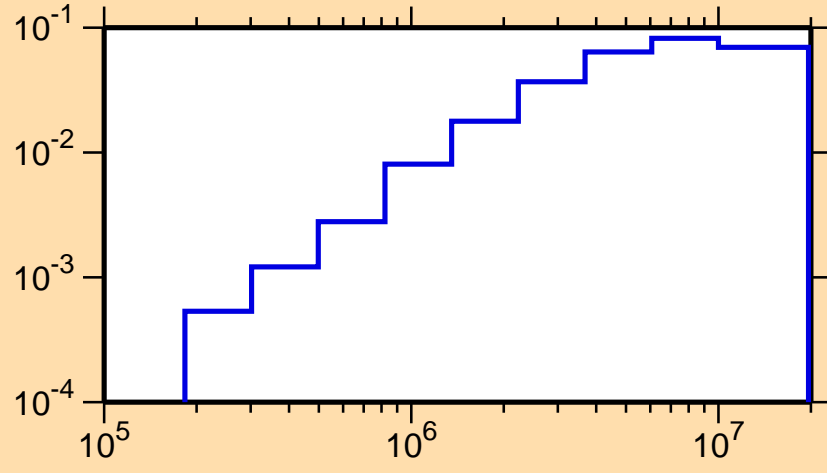
\sigma vs. E for ^{140}\text{Tb}(n,\text{inel.})
