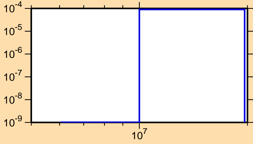
\sigma vs. E for ^{140}\text{Tb}(\text{mt } 45)
