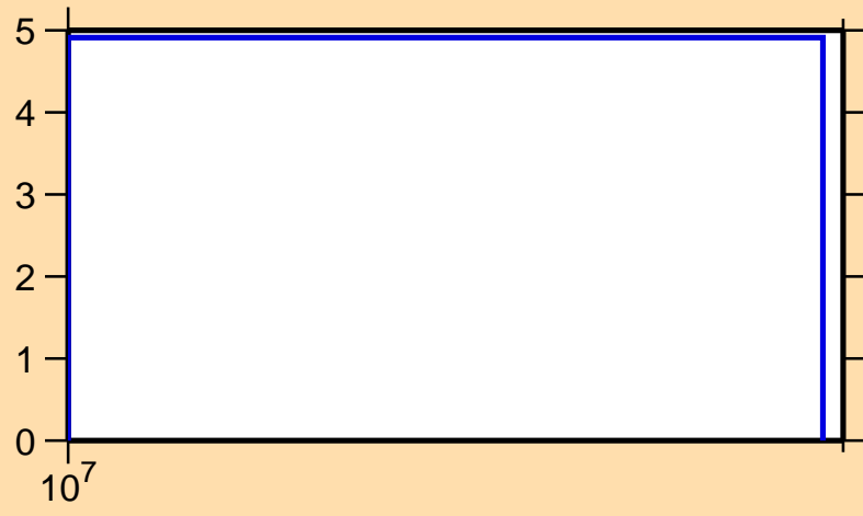
\Delta\sigma/\sigma vs. E for ^{140}\text{Tb}(n,\text{nonel.})
