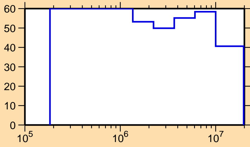
\Delta\sigma/\sigma vs. E for ^{140}\text{Tb}(n,n_1)
