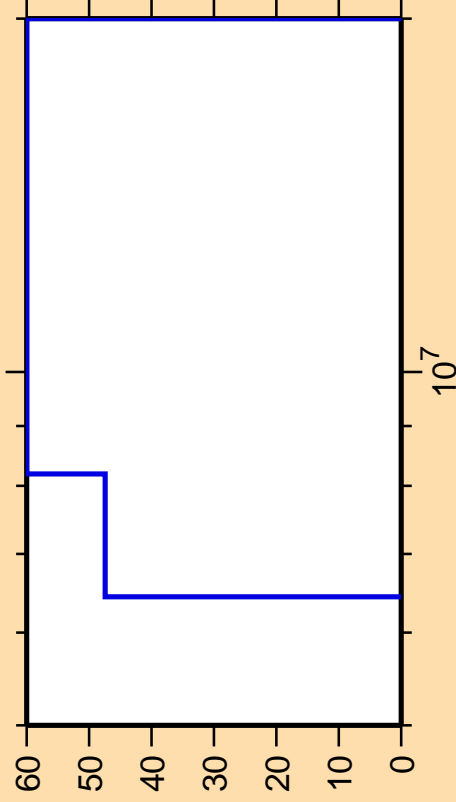
\Delta\sigma/\sigma vs. E for ^{140}\text{Tb} (mt 45)
