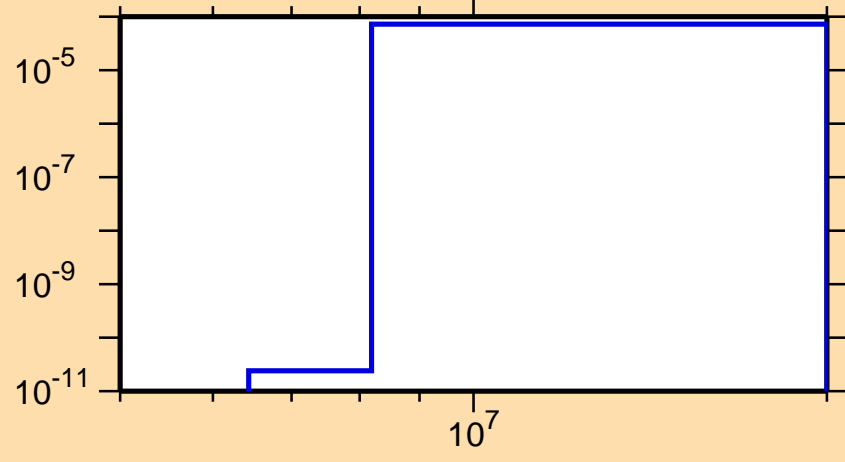
\sigma vs. E for ^{140}\text{Tb} (mt 45)
