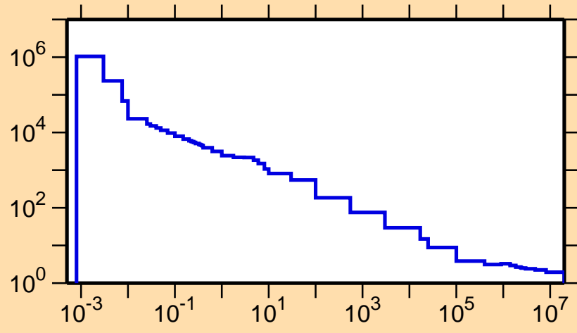
\sigma vs. E for ^{140}\text{Tb}(n,\text{nonel.})
