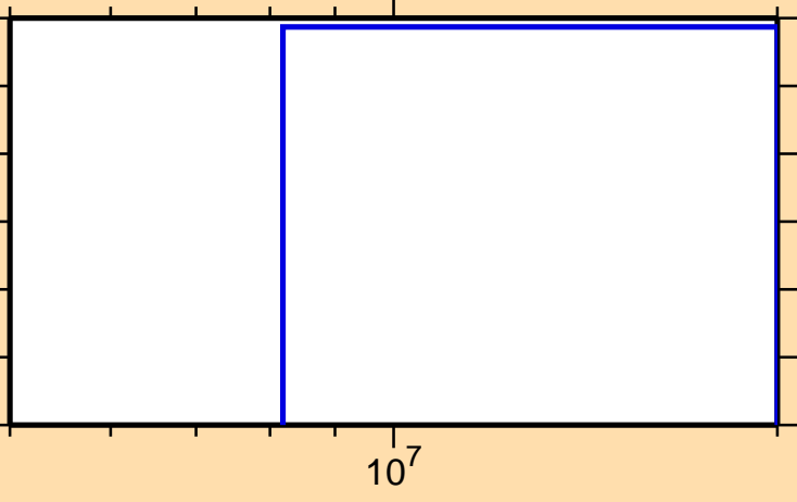
\sigma vs. E for ^{140}\text{Tb}(n,\text{nd})
