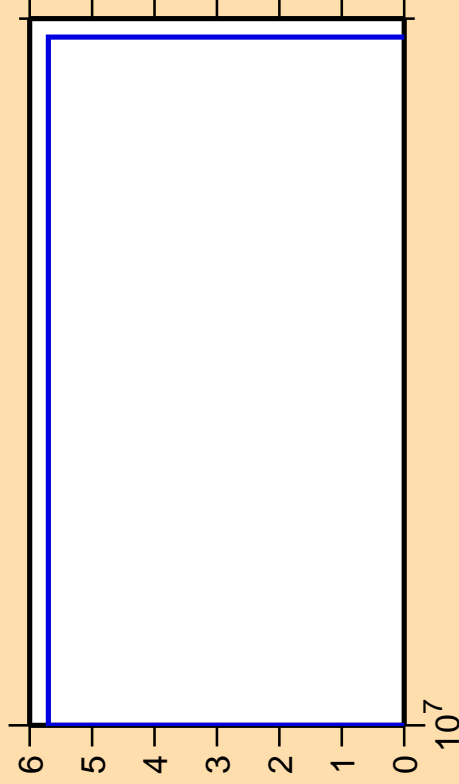
\Delta\sigma/\sigma vs. E for ^{141}\text{Tb}(n,nt)
