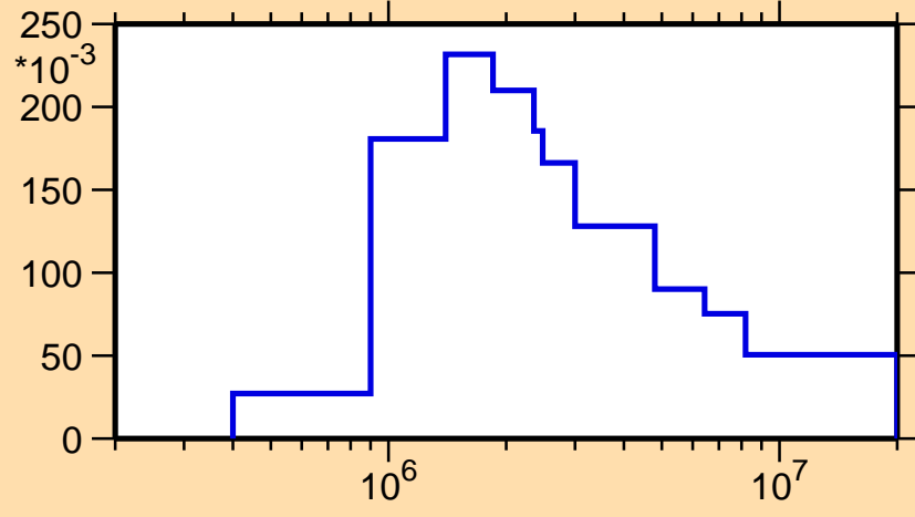
\sigma vs. E for ^{141}\text{Tb}(n,n_3)
