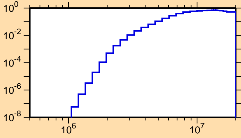
\sigma vs. E for ^{141}\text{Tb}(n,np)
