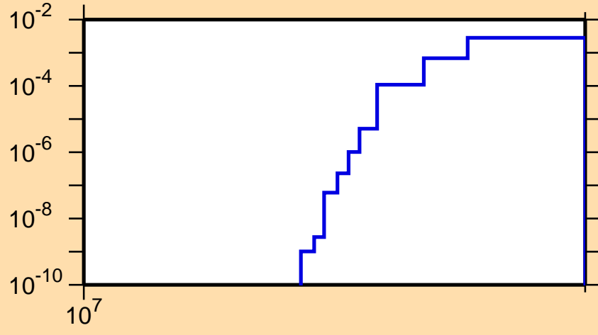
\sigma vs. E for ^{141}\text{Tb}(n,2np)
