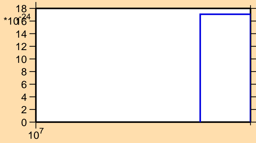
\sigma vs. E for ^{141}\text{Tb} (mt 11)
