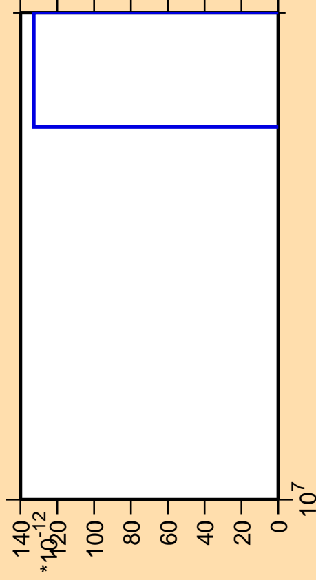
\Delta\sigma/\sigma vs. E for ^{141}\text{Tb} (mt 11)
