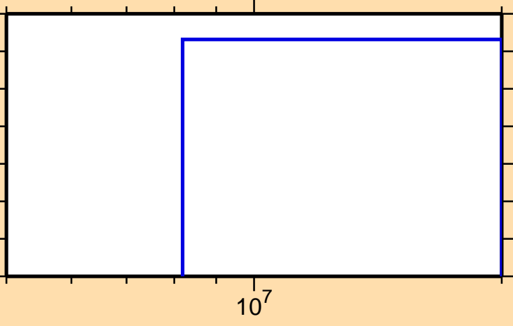
\sigma vs. E for ^{141}\text{Tb}(n,2np)
