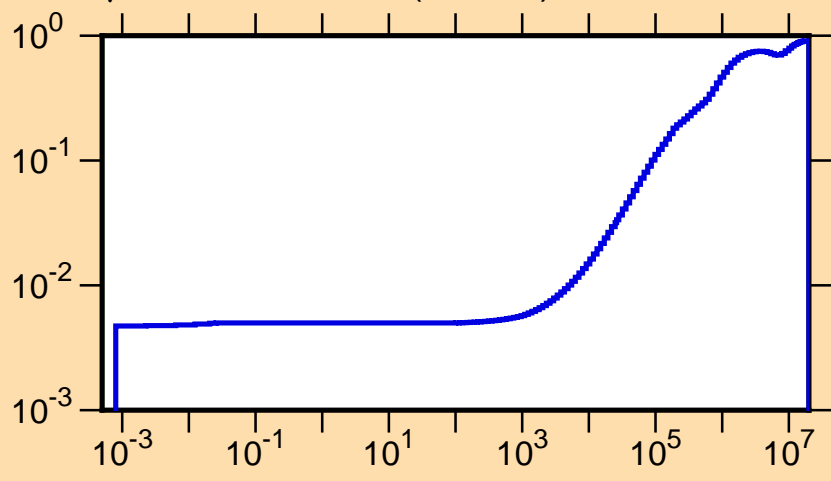
\mu vs. E for ^{143}\text{Tb}(\text{mt251})
