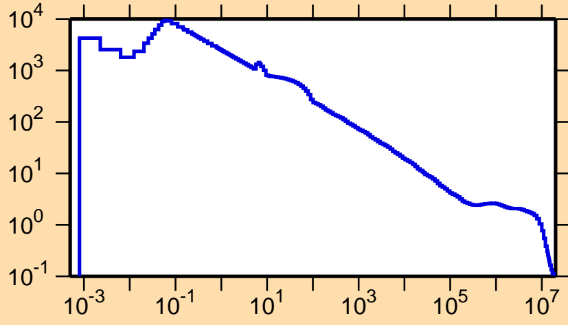
\sigma vs. E for ^{143}\text{Tb}(n,p)
