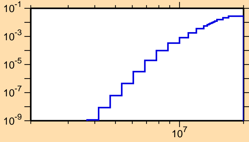
\sigma vs. E for ^{143}\text{Tb}(n,n\alpha)
