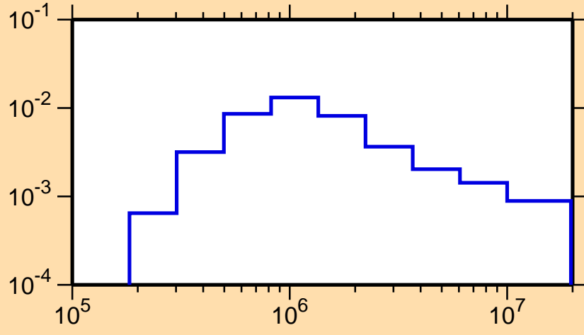
\sigma vs. E for ^{143}\text{Tb}(n,n_2)
