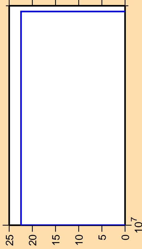
\Delta\sigma/\sigma vs. E for ^{143}\text{Tb} (mt 34)
