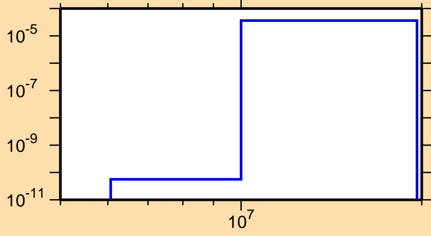
\sigma vs. E for ^{143}\text{Tb} (mt 45)
