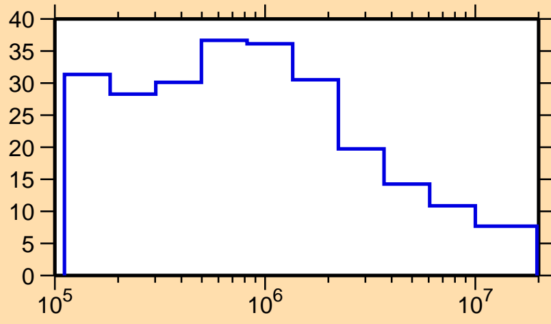
\Delta\sigma/\sigma vs. E for ^{143}\text{Tb}(n,\text{nonel.})
