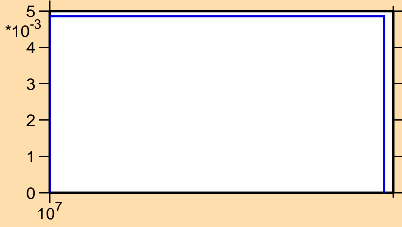
\sigma vs. E for ^{143}\text{Tb}(n,2n)
