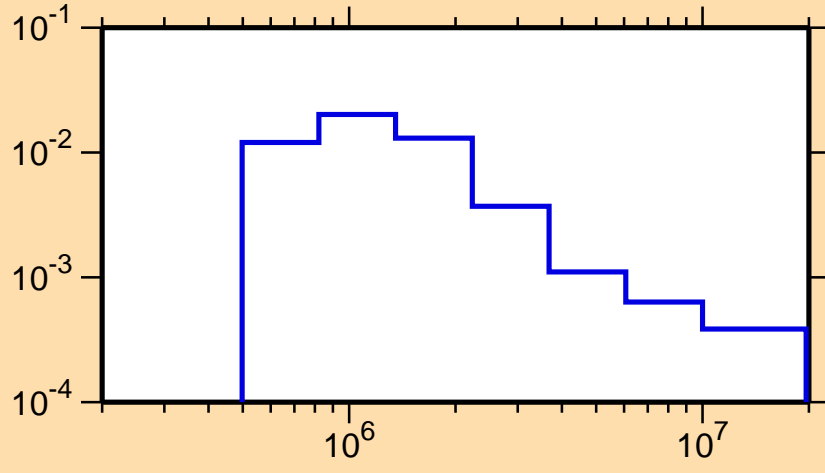
\sigma vs. E for ^{143}\text{Tb}(n,n_4)
