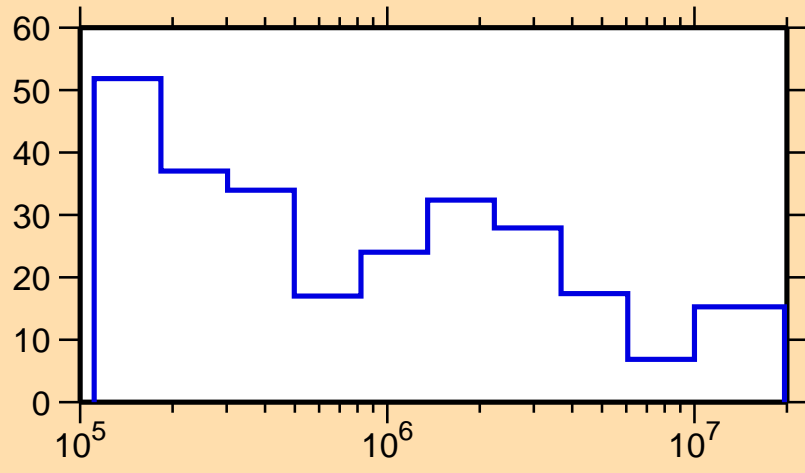
\Delta\sigma/\sigma vs. E for ^{143}\text{Tb}(n,\text{tot.})
