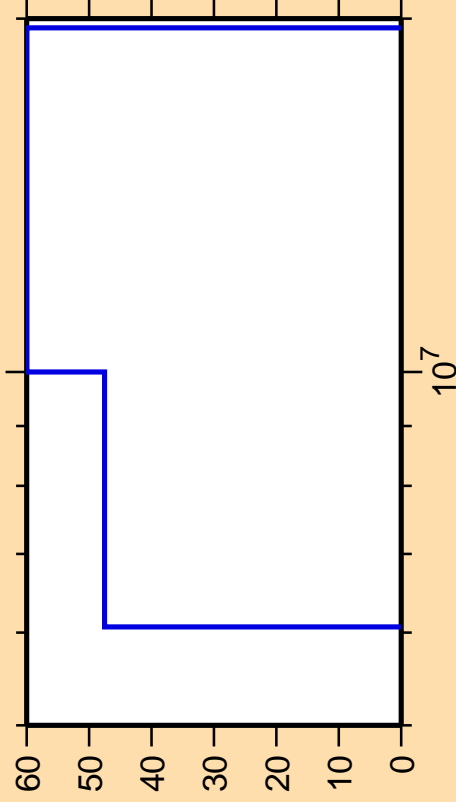
\Delta\sigma/\sigma vs. E for ^{143}\text{Tb} (mt 45)
