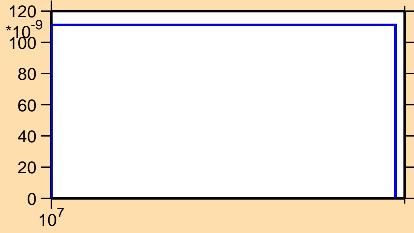
\sigma vs. E for ^{143}\text{Tb}(n,\text{nd})
