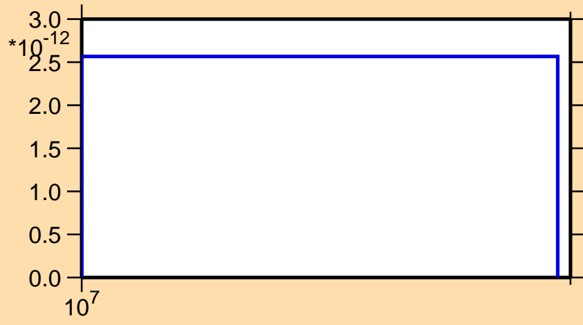
\sigma vs. E for ^{143}\text{Tb} (mt 34)
