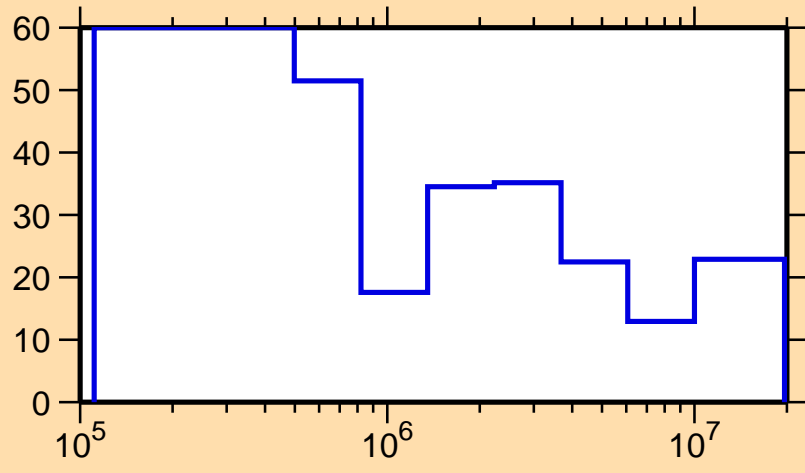
\Delta\sigma/\sigma vs. E for ^{143}\text{Tb}(n,\text{el.})
