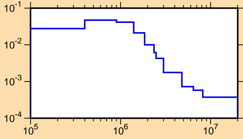
\sigma vs. E for ^{143}\text{Tb}(n,n_1)
