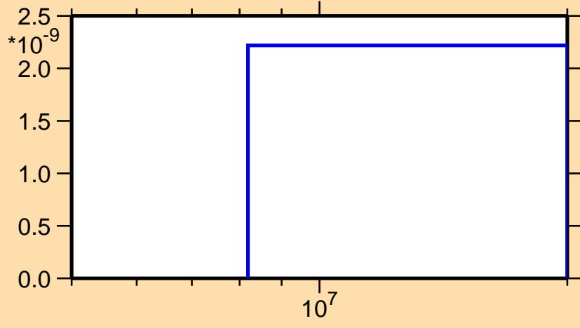
\sigma vs. E for ^{143}\text{Tb}(n,\text{pt})
