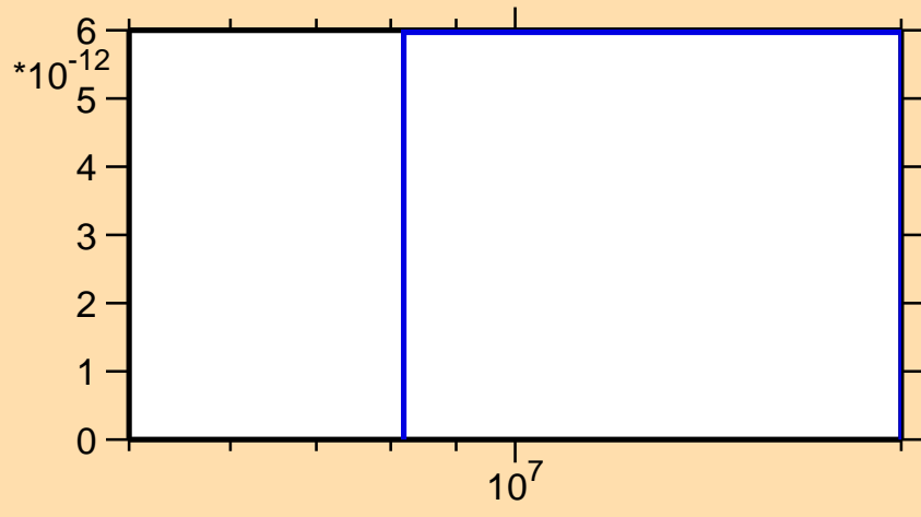
\sigma vs. E for ^{143}\text{Tb}(n,nt)
