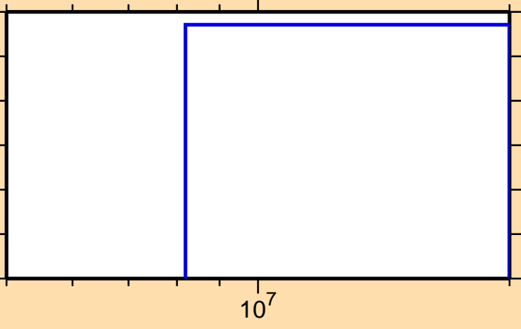
\sigma vs. E for ^{143}\text{Tb}(n,pd)
