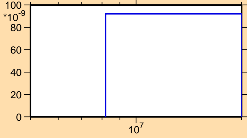
\sigma vs. E for ^{143}\text{Tb}(n,\text{nd})
