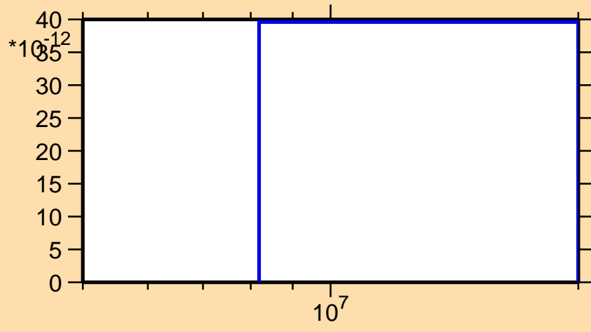
\sigma vs. E for ^{143}\text{Tb}(n,2n\alpha)
