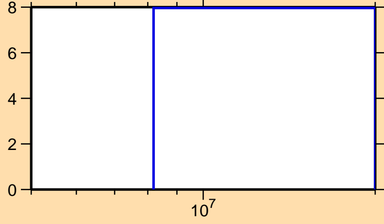
\Delta\sigma/\sigma vs. E for ^{143}\text{Tb}(n,\text{nonel.})
