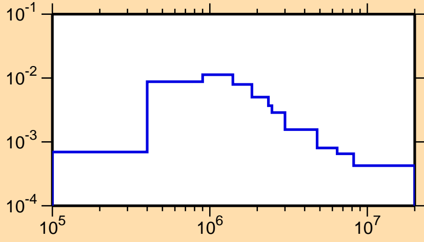
\sigma vs. E for ^{143}\text{Tb}(n,n_3)
