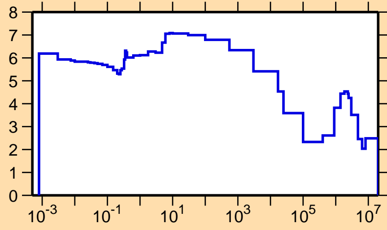
\sigma vs. E for ^{143}\text{Tb}(n,\text{el.})
