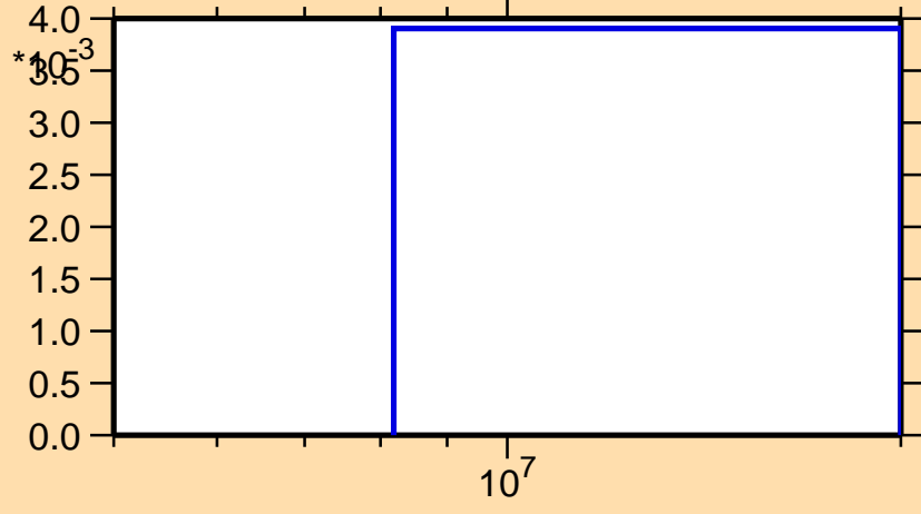
\sigma vs. E for ^{143}\text{Tb}(n,2n)
