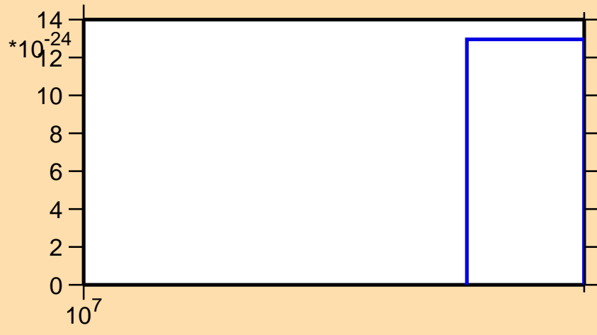
\sigma vs. E for ^{143}\text{Tb} (mt 11)
