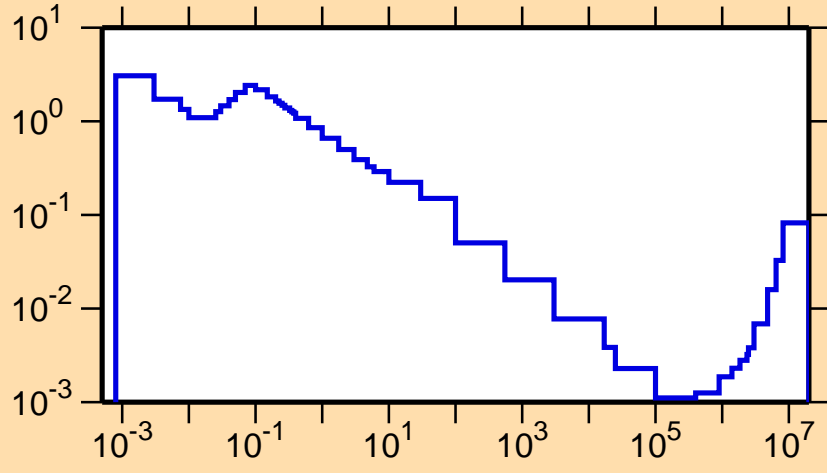
\sigma vs. E for ^{143}\text{Tb}(n,\alpha)
