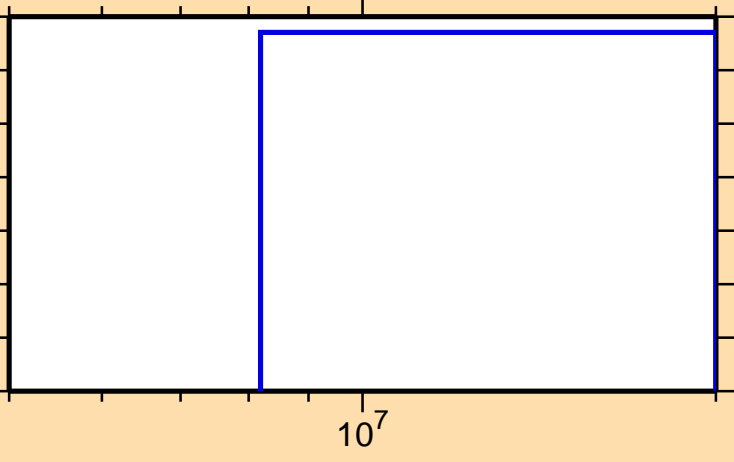
\sigma vs. E for ^{143}\text{Tb}(n,\text{pt})
