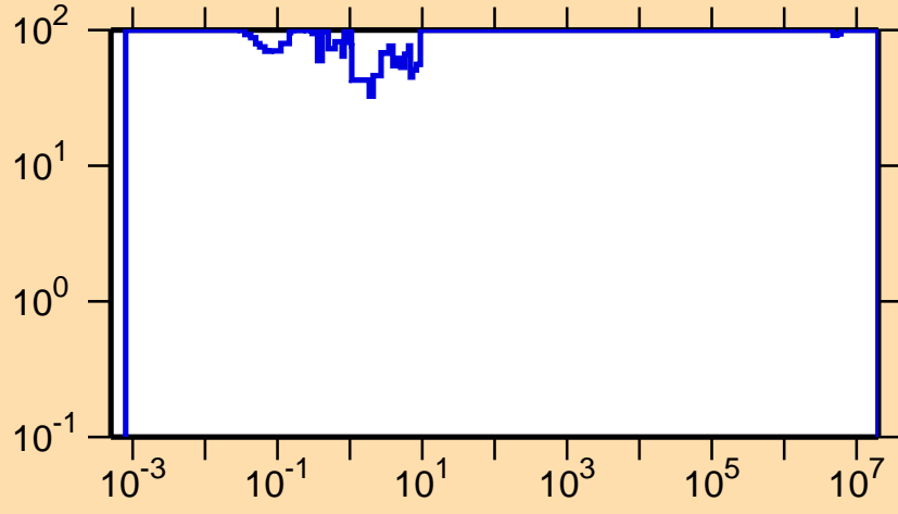
\Delta\sigma/\sigma vs. E for ^{144}\text{Tb}(n,\gamma)
