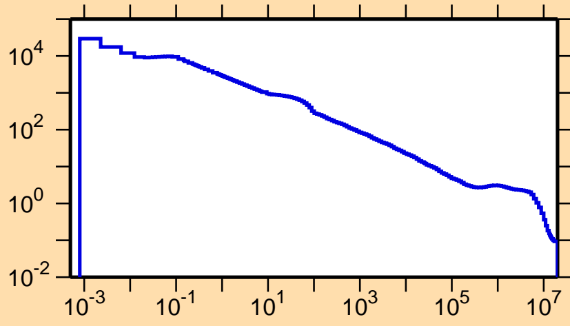
\sigma vs. E for ^{144}\text{Tb}(n,p)
