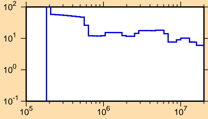
\Delta\sigma/\sigma vs. E for ^{144}\text{Tb}(n,\text{el.})
