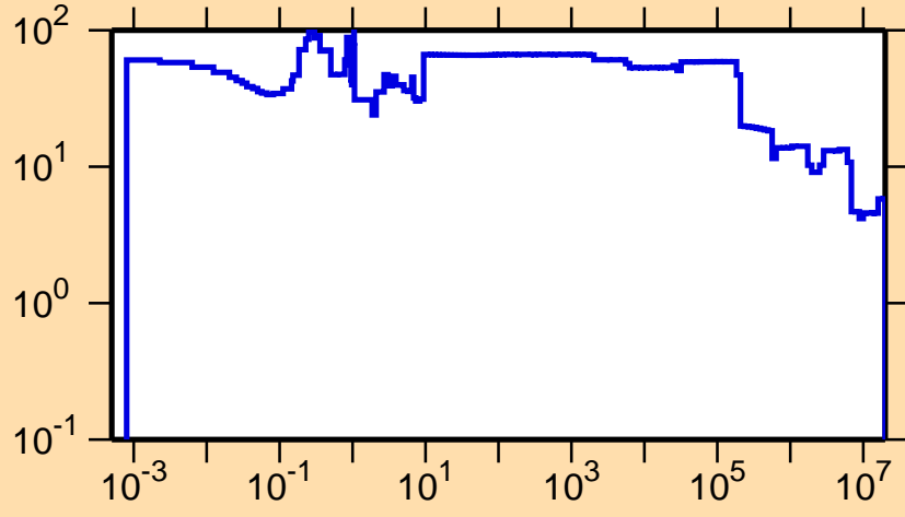
\Delta\sigma/\sigma vs. E for ^{144}\text{Tb}(n,\text{tot.})
