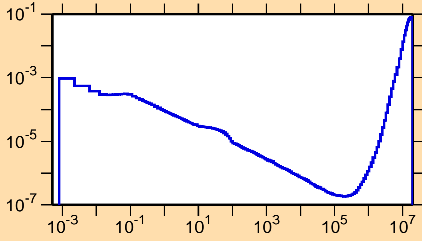
\sigma vs. E for ^{144}\text{Tb}(n,p\alpha)
