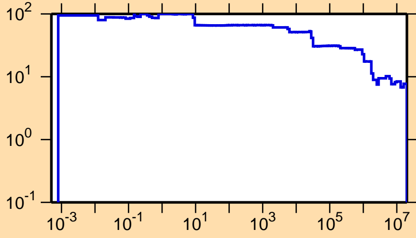
\Delta\sigma/\sigma vs. E for ^{144}\text{Tb}(n,\text{nonel.})
