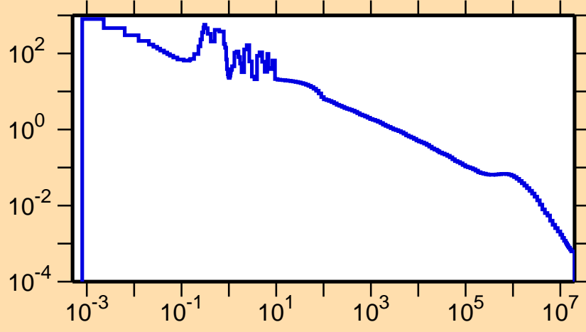
\sigma vs. E for ^{144}\text{Tb}(n,\gamma)
