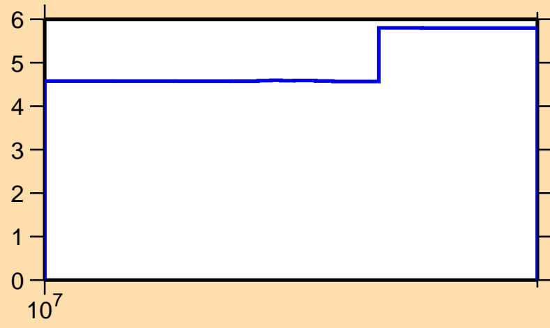
\Delta\sigma/\sigma vs. E for ^{144}\text{Tb}(n,\text{tot.})
