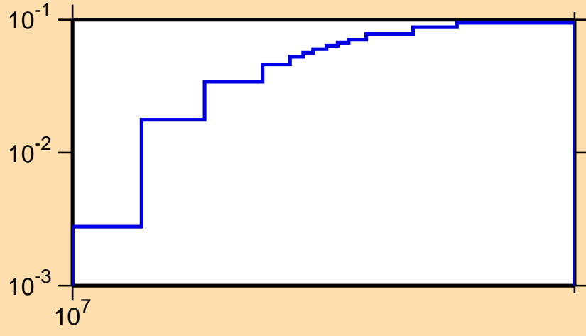
\sigma vs. E for ^{144}\text{Tb}(n,2n)
