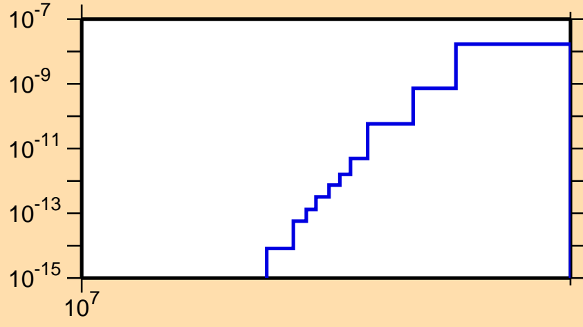
\sigma vs. E for ^{144}\text{Tb} (mt 34)
