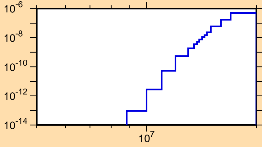
\sigma vs. E for ^{144}\text{Tb}(\text{mt117})
