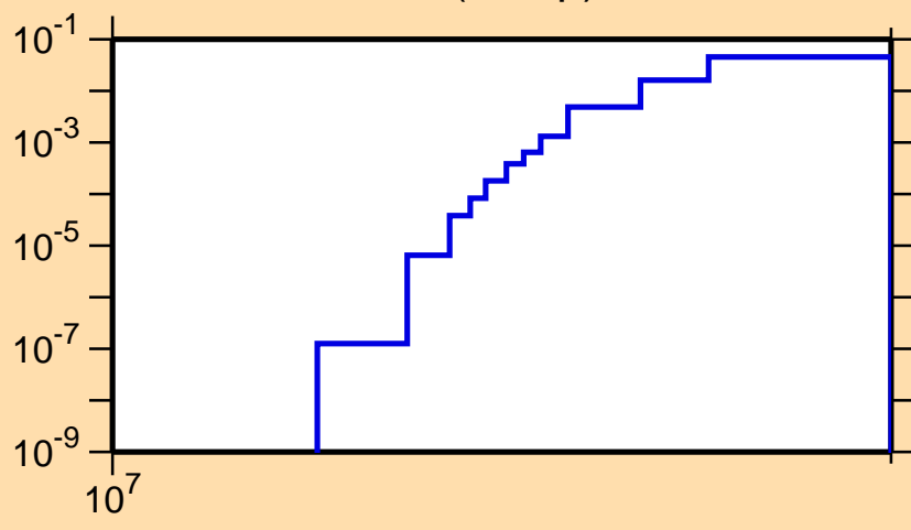
\sigma vs. E for ^{144}\text{Tb}(n,2np)
