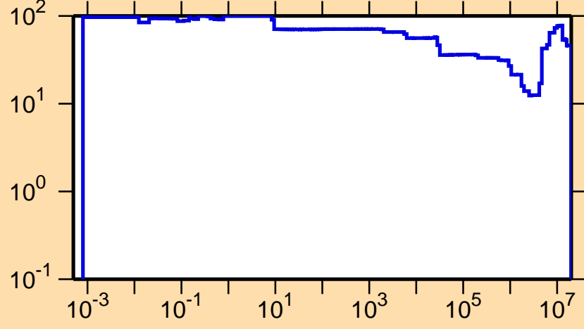
\Delta\sigma/\sigma vs. E for ^{144}\text{Tb}(n,p)
