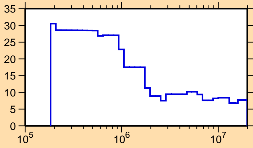
\Delta\sigma/\sigma vs. E for ^{144}\text{Tb}(n,\text{nonel.})
