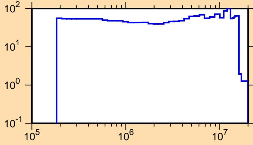
\Delta\sigma/\sigma vs. E for ^{144}\text{Tb}(n,n_1)
