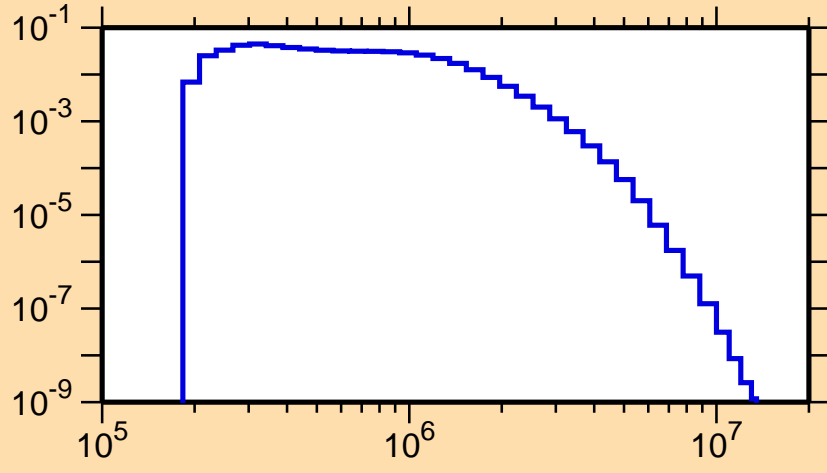
\sigma vs. E for ^{144}\text{Tb}(n,n_1)
