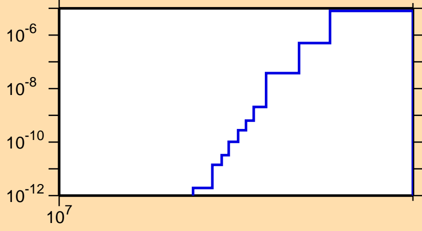
\sigma vs. E for ^{144}\text{Tb}(n,\text{pt})
